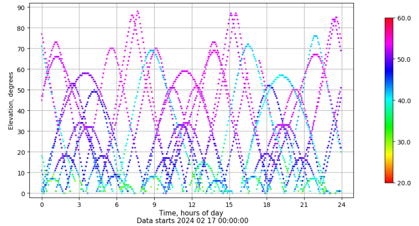
Time-elevation plot for station SALA. Signal to Noise S1C Data file SALA00ESP_R_2024048.xtr
