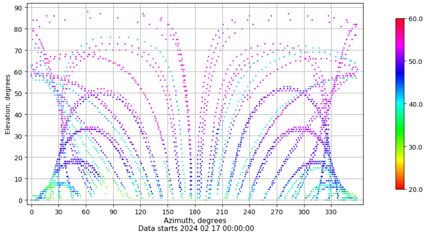
Azimuth-elevation plot for station SALA. Signal to Noise S1C Data file SALA00ESP_R_2024048.xtr
