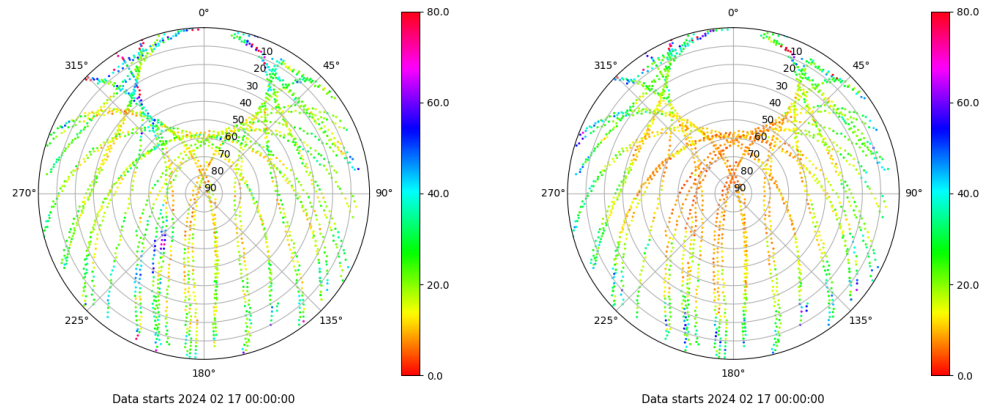
Skyplot for station SALA. Parameter M1C Data file SALA00ESP_R_2024048.xtr Skyplot for station SALA. Parameter M2P Data file SALA00ESP_R_2024048.xtr
