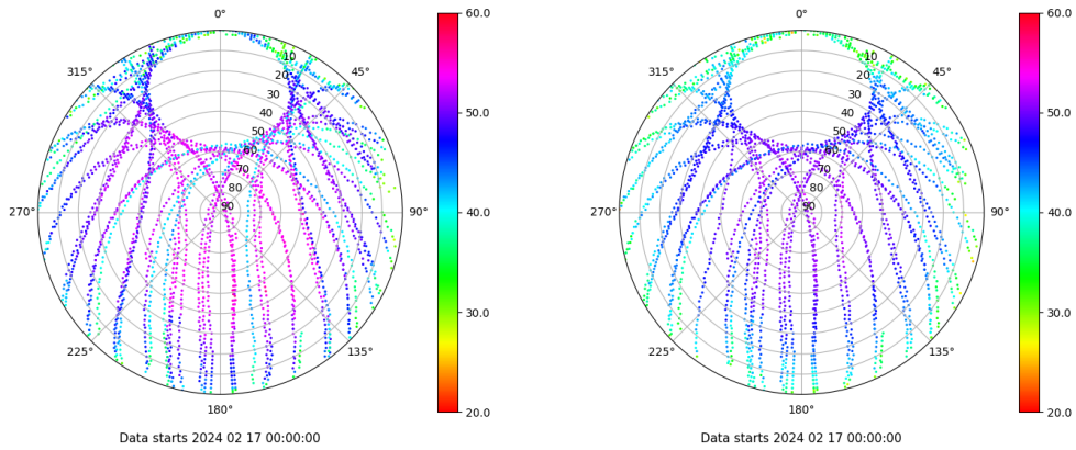
Skyplot for station SALA. Signal to Noise S1C Data file SALA00ESP_R_2024048.xtr Skyplot for station SALA. Signal to Noise S2P Data file SALA00ESP_R_2024048.xtr
