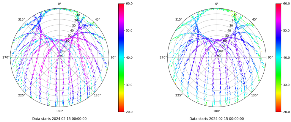
Skyplot for station SALA. Signal to Noise S1C Data file SALA00ESP_R_2024046.xtr Skyplot for station SALA. Signal to Noise S2P Data file SALA00ESP_R_2024046.xtr
