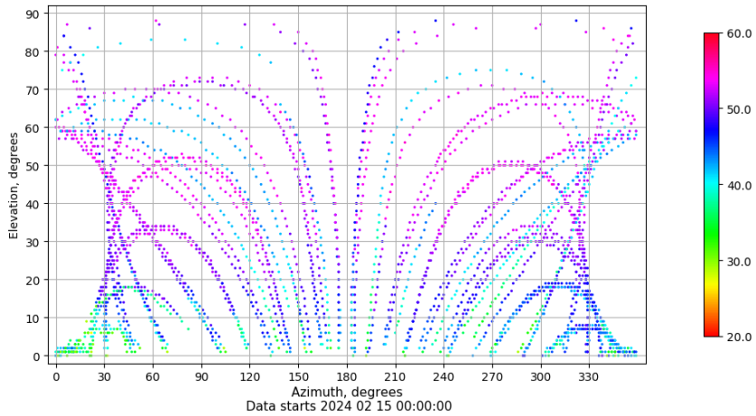
Azimuth-elevation plot for station SALA. Signal to Noise S1C Data file SALA00ESP_R_2024046.xtr
