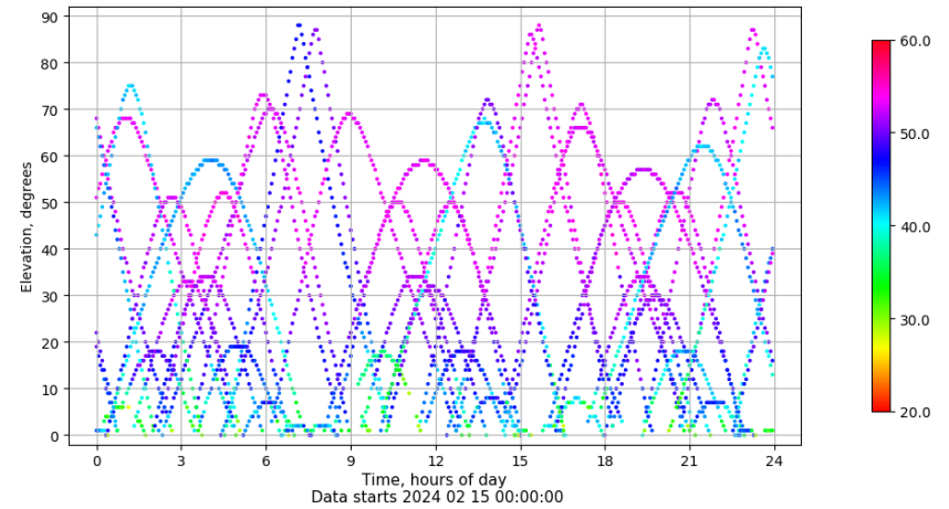
Time-elevation plot for station SALA. Signal to Noise S1C Data file SALA00ESP_R_2024046.xtr
