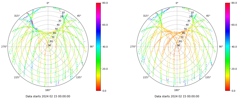
Skyplot for station SALA. Parameter M1C Data file SALA00ESP_R_2024046.xtr Skyplot for station SALA. Parameter M2P Data file SALA00ESP_R_2024046.xtr
