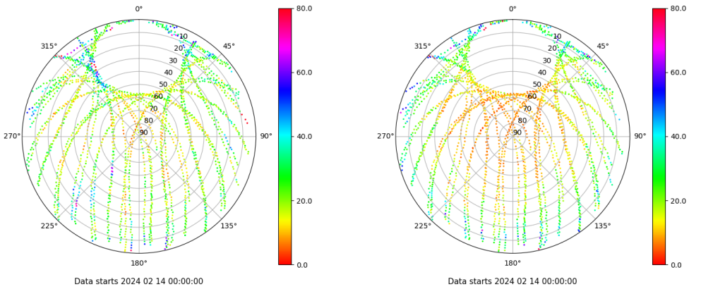
Skyplot for station SALA. Parameter M1C Data file SALA00ESP_R_2024045.xtr Skyplot for station SALA. Parameter M2P Data file SALA00ESP_R_2024045.xtr
