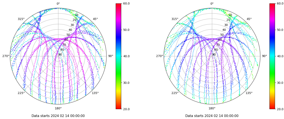
Skyplot for station SALA. Signal to Noise S1C Data file SALA00ESP_R_2024045.xtr Skyplot for station SALA. Signal to Noise S2P Data file SALA00ESP_R_2024045.xtr
