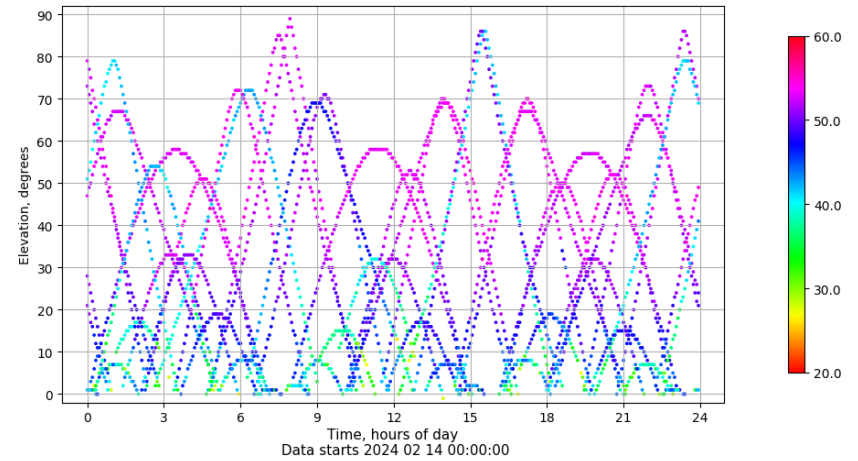
Time-elevation plot for station SALA. Signal to Noise S1C Data file SALA00ESP_R_2024045.xtr
