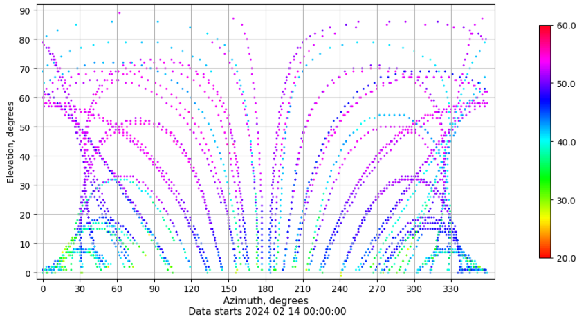
Azimuth-elevation plot for station SALA. Signal to Noise S1C Data file SALA00ESP_R_2024045.xtr
