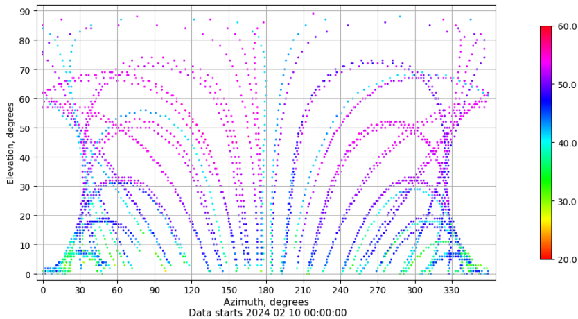
Azimuth-elevation plot for station SALA. Signal to Noise S1C Data file SALA00ESP_R_2024041.xtr
