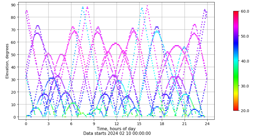
Time-elevation plot for station SALA. Signal to Noise S1C Data file SALA00ESP_R_2024041.xtr
