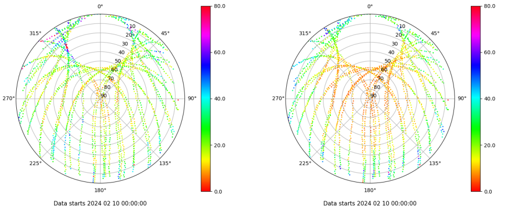
Skyplot for station SALA. Parameter M1C Data file SALA00ESP_R_2024041.xtr Skyplot for station SALA. Parameter M2P Data file SALA00ESP_R_2024041.xtr
