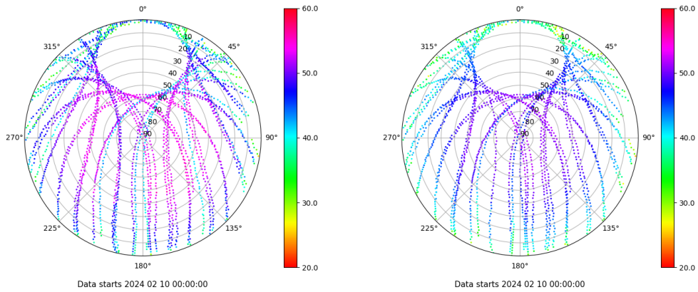
Skyplot for station SALA. Signal to Noise S1C Data file SALA00ESP_R_2024041.xtr Skyplot for station SALA. Signal to Noise S2P Data file SALA00ESP_R_2024041.xtr
