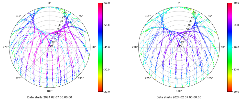
Skyplot for station SALA. Signal to Noise S1C Data file SALA00ESP_R_2024038.xtr Skyplot for station SALA. Signal to Noise S2P Data file SALA00ESP_R_2024038.xtr
