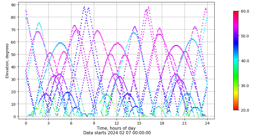
Time-elevation plot for station SALA. Signal to Noise S1C Data file SALA00ESP_R_2024038.xtr
