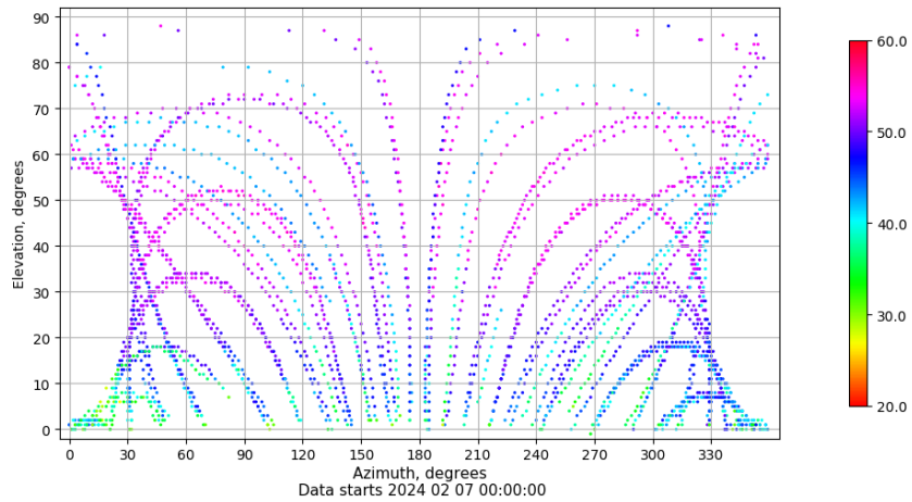
Azimuth-elevation plot for station SALA. Signal to Noise S1C Data file SALA00ESP_R_2024038.xtr
