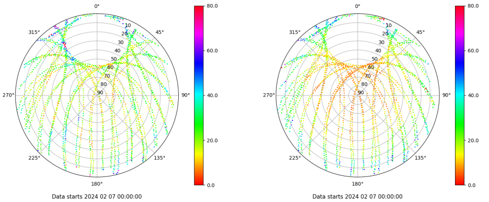
Skyplot for station SALA. Parameter M1C Data file SALA00ESP_R_2024038.xtr Skyplot for station SALA. Parameter M2P Data file SALA00ESP_R_2024038.xtr
