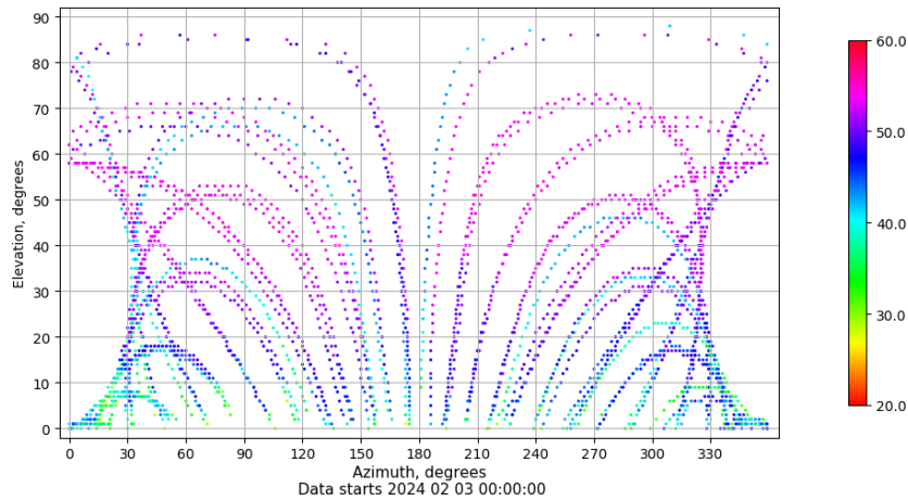
Azimuth-elevation plot for station SALA. Signal to Noise S1C Data file SALA00ESP_R_2024034.xtr
