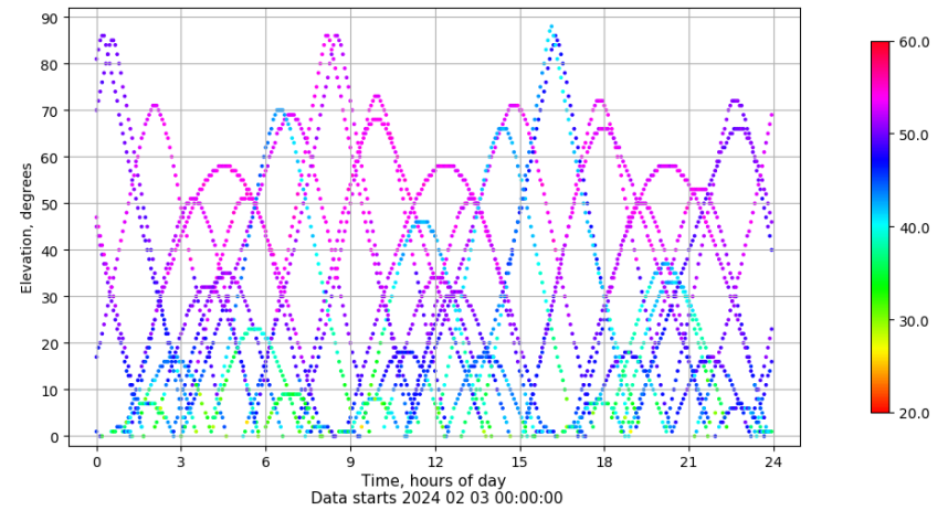
Time-elevation plot for station SALA. Signal to Noise S1C Data file SALA00ESP_R_2024034.xtr
