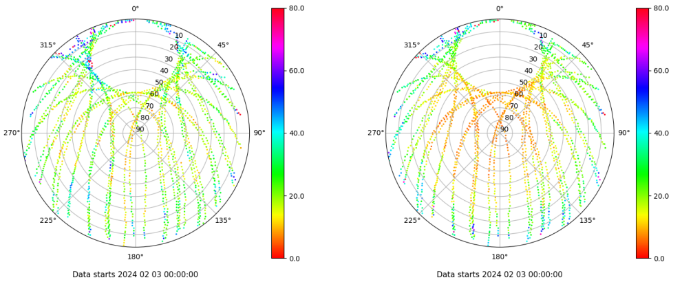
Skyplot for station SALA. Parameter M1C Data file SALA00ESP_R_2024034.xtr Skyplot for station SALA. Parameter M2P Data file SALA00ESP_R_2024034.xtr
