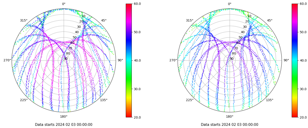
Skyplot for station SALA. Signal to Noise S1C Data file SALA00ESP_R_2024034.xtr Skyplot for station SALA. Signal to Noise S2P Data file SALA00ESP_R_2024034.xtr
