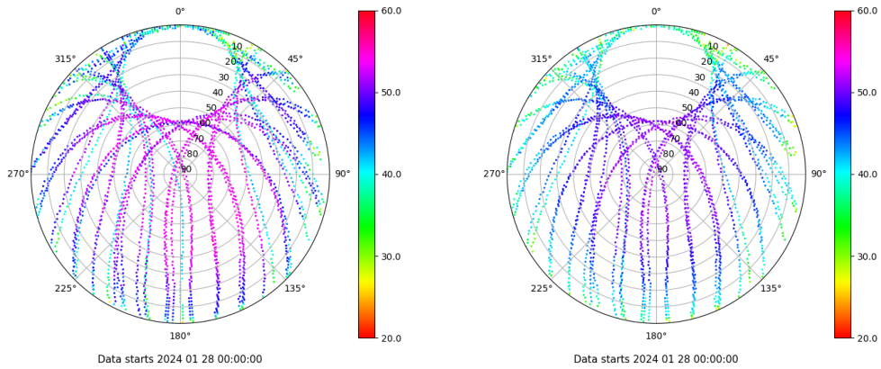
Skyplot for station SALA. Signal to Noise S1C Data file SALA00ESP_R_2024028.xtr Skyplot for station SALA. Signal to Noise S2P Data file SALA00ESP_R_2024028.xtr
