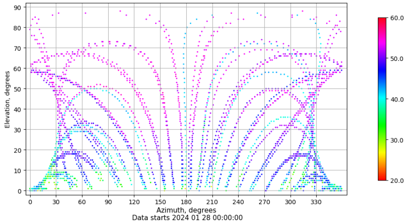
Azimuth-elevation plot for station SALA. Signal to Noise S1C Data file SALA00ESP_R_2024028.xtr
