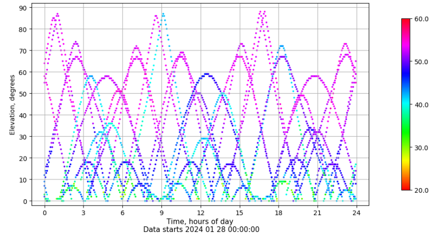
Time-elevation plot for station SALA. Signal to Noise S1C Data file SALA00ESP_R_2024028.xtr
