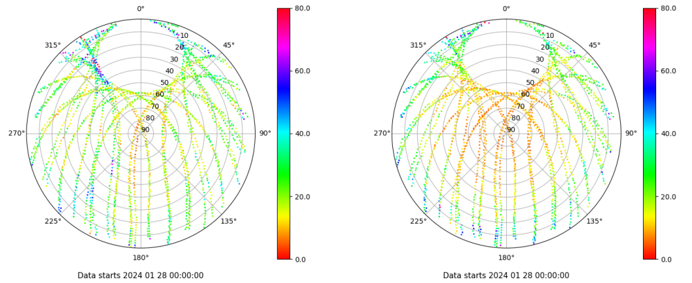
Skyplot for station SALA. Parameter M1C Data file SALA00ESP_R_2024028.xtr Skyplot for station SALA. Parameter M2P Data file SALA00ESP_R_2024028.xtr
