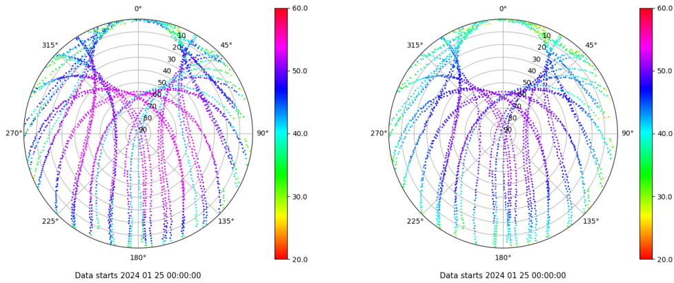
Skyplot for station SALA. Signal to Noise S1C Data file SALA00ESP_R_2024025.xtr Skyplot for station SALA. Signal to Noise S2P Data file SALA00ESP_R_2024025.xtr
