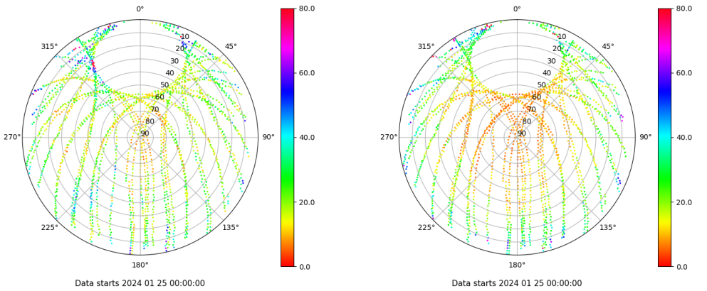
Skyplot for station SALA. Parameter M1C Data file SALA00ESP_R_2024025.xtr Skyplot for station SALA. Parameter M2P Data file SALA00ESP_R_2024025.xtr
