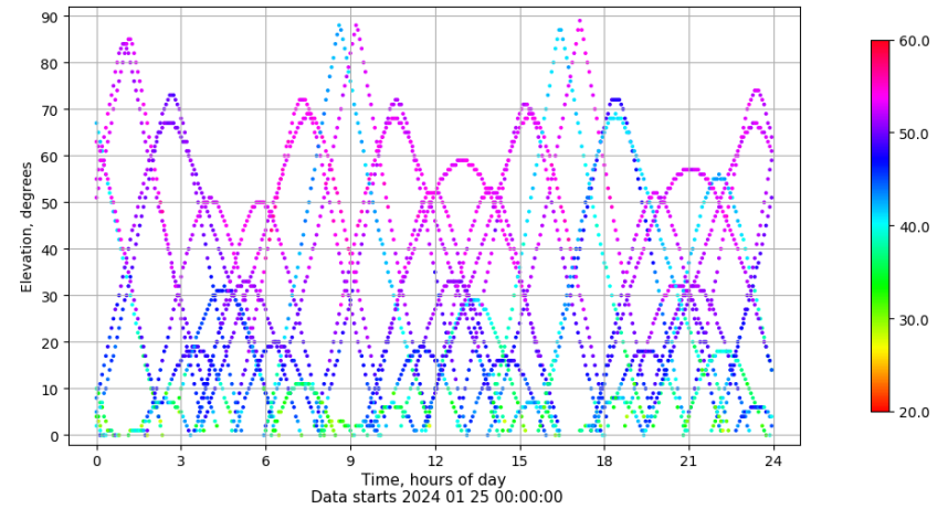
Time-elevation plot for station SALA. Signal to Noise S1C Data file SALA00ESP_R_2024025.xtr
