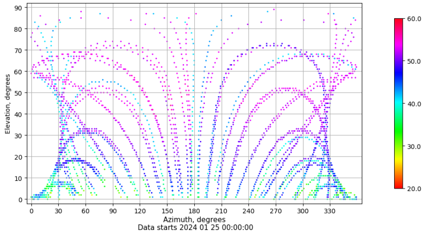
Azimuth-elevation plot for station SALA. Signal to Noise S1C Data file SALA00ESP_R_2024025.xtr
