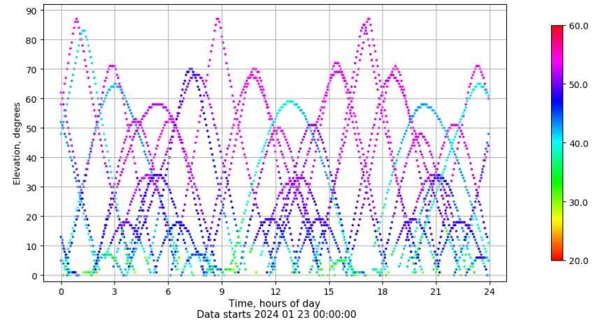
Time-elevation plot for station SALA. Signal to Noise S1C Data file SALA00ESP_R_2024023.xtr
