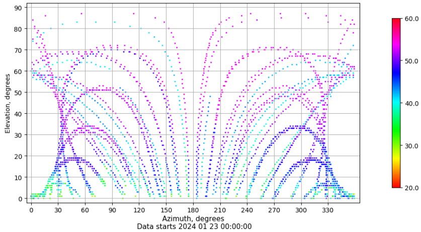
Azimuth-elevation plot for station SALA. Signal to Noise S1C Data file SALA00ESP_R_2024023.xtr
