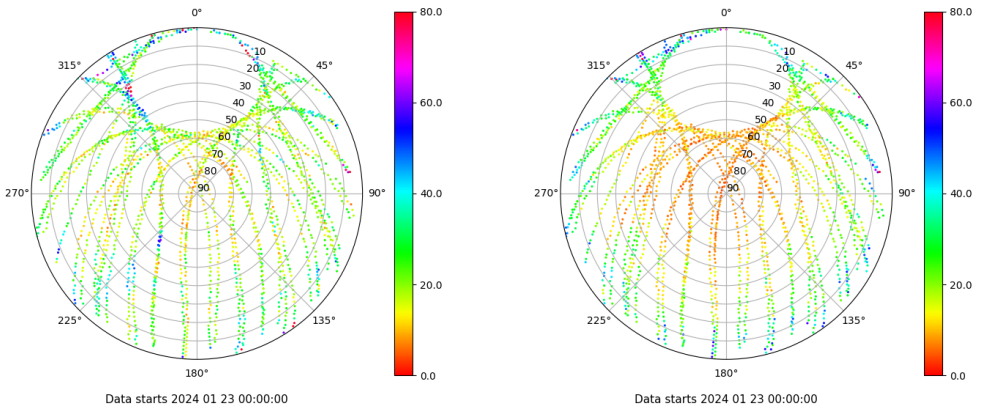
Skyplot for station SALA. Parameter M1C Data file SALA00ESP_R_2024023.xtr Skyplot for station SALA. Parameter M2P Data file SALA00ESP_R_2024023.xtr
