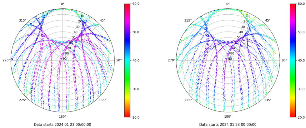
Skyplot for station SALA. Signal to Noise S1C Data file SALA00ESP_R_2024023.xtr Skyplot for station SALA. Signal to Noise S2P Data file SALA00ESP_R_2024023.xtr
