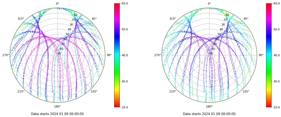
Skyplot for station SALA. Signal to Noise S1C Data file SALA00ESP_R_2024009.xtr Skyplot for station SALA. Signal to Noise S2P Data file SALA00ESP_R_2024009.xtr
