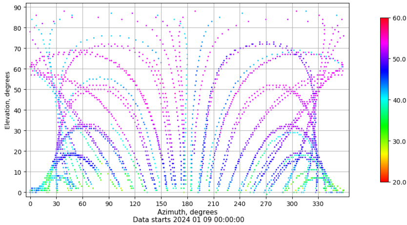
Azimuth-elevation plot for station SALA. Signal to Noise S1C Data file SALA00ESP_R_2024009.xtr
