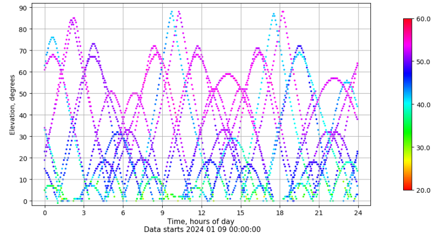
Time-elevation plot for station SALA. Signal to Noise S1C Data file SALA00ESP_R_2024009.xtr
