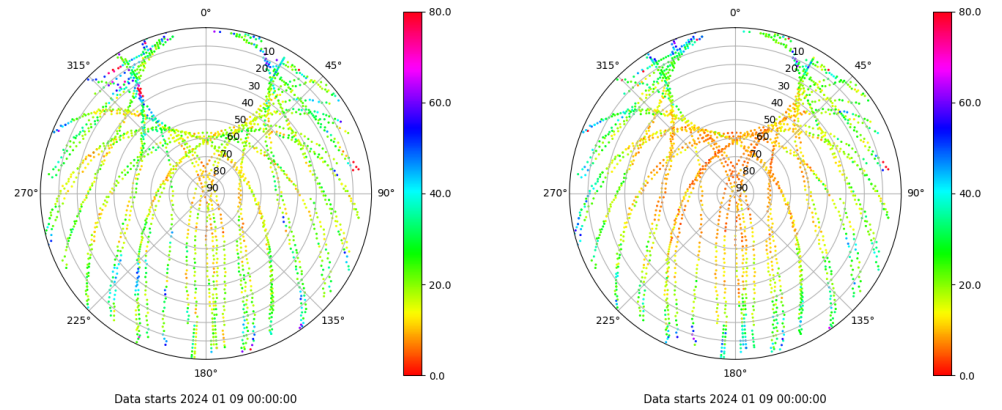
Skyplot for station SALA. Parameter M1C Data file SALA00ESP_R_2024009.xtr Skyplot for station SALA. Parameter M2P Data file SALA00ESP_R_2024009.xtr
