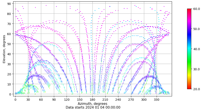
Azimuth-elevation plot for station SALA. Signal to Noise S1C Data file SALA00ESP_R_2024004.xtr
