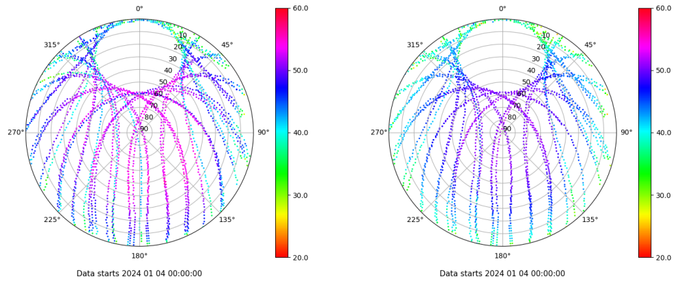
Skyplot for station SALA. Signal to Noise S1C Data file SALA00ESP_R_2024004.xtr Skyplot for station SALA. Signal to Noise S2P Data file SALA00ESP_R_2024004.xtr
