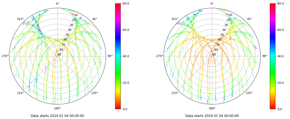
Skyplot for station SALA. Parameter M1C Data file SALA00ESP_R_2024004.xtr Skyplot for station SALA. Parameter M2P Data file SALA00ESP_R_2024004.xtr
