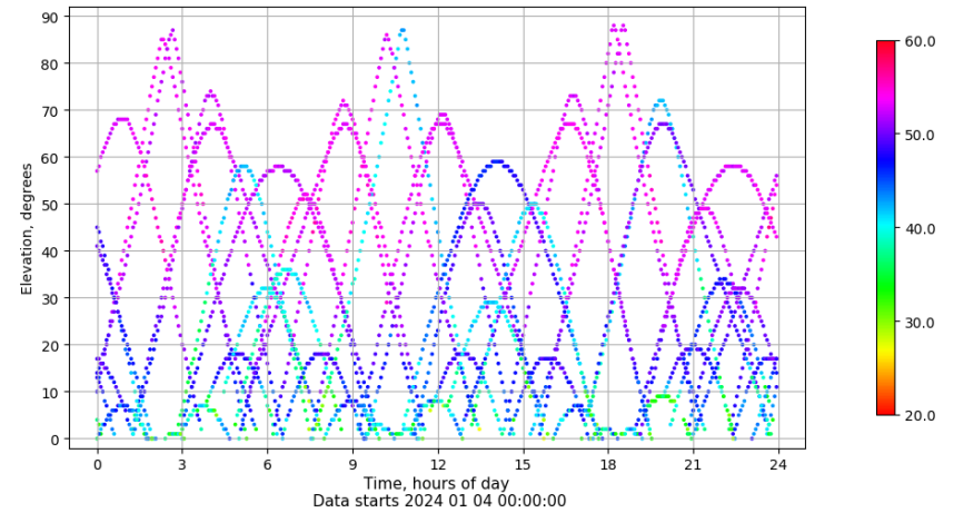
Time-elevation plot for station SALA. Signal to Noise S1C Data file SALA00ESP_R_2024004.xtr
