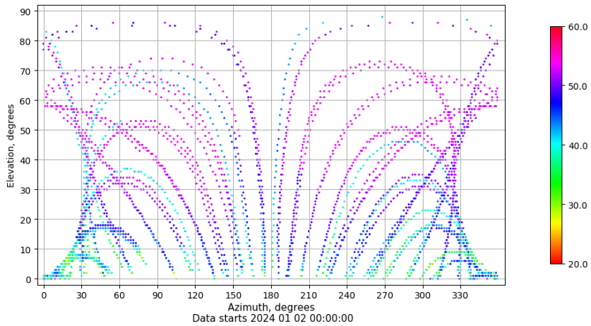
Azimuth-elevation plot for station SALA. Signal to Noise S1C Data file SALA00ESP_R_2024002.xtr
