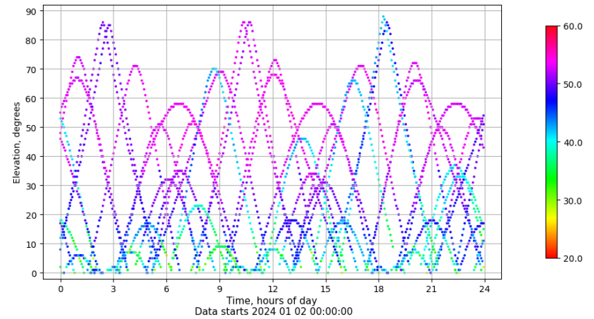
Time-elevation plot for station SALA. Signal to Noise S1C Data file SALA00ESP_R_2024002.xtr
