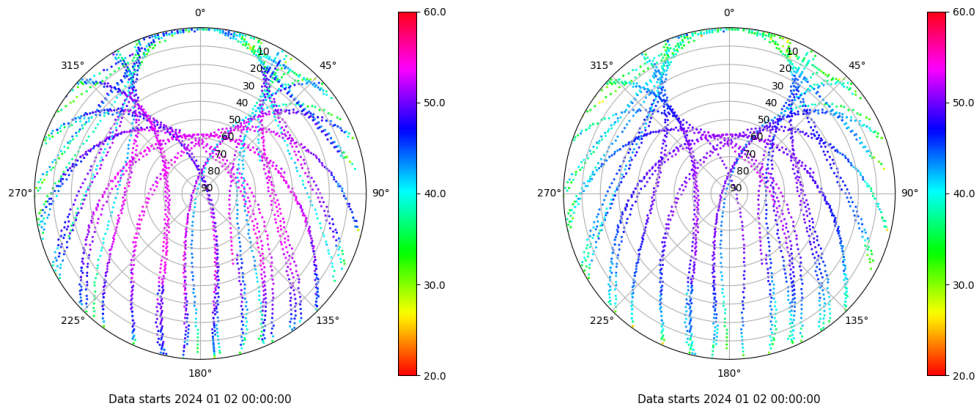
Skyplot for station SALA. Signal to Noise S1C Data file SALA00ESP_R_2024002.xtr Skyplot for station SALA. Signal to Noise S2P Data file SALA00ESP_R_2024002.xtr
