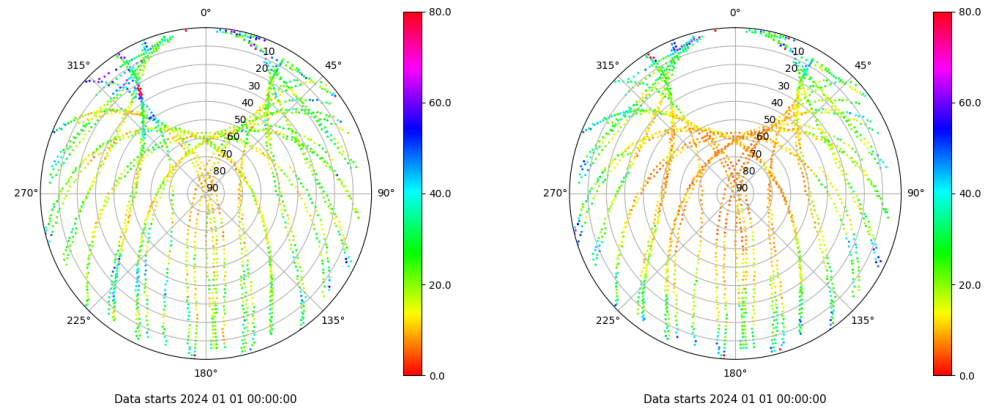
Skyplot for station SALA. Parameter M1C Data file SALA00ESP_R_2024001.xtr Skyplot for station SALA. Parameter M2P Data file SALA00ESP_R_2024001.xtr
