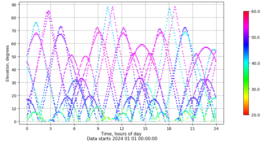
Time-elevation plot for station SALA. Signal to Noise S1C Data file SALA00ESP_R_2024001.xtr
