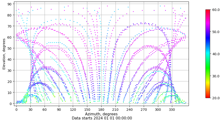
Azimuth-elevation plot for station SALA. Signal to Noise S1C Data file SALA00ESP_R_2024001.xtr
