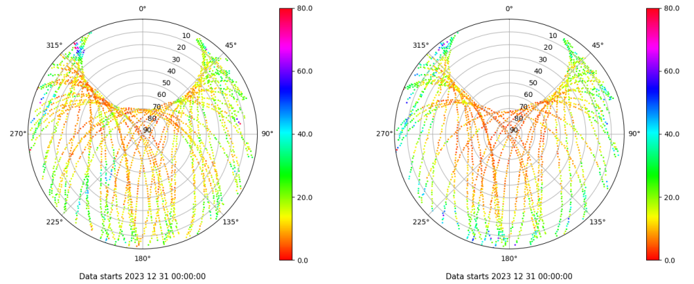
Skyplot for station SALA. Parameter M1C Data file SALA00ESP_R_2023365.xtr Skyplot for station SALA. Parameter M2S Data file SALA00ESP_R_2023365.xtr
