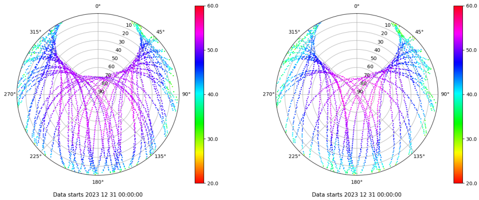
Skyplot for station SALA. Signal to Noise S1C Data file SALA00ESP_R_2023365.xtr Skyplot for station SALA. Signal to Noise S2S Data file SALA00ESP_R_2023365.xtr
