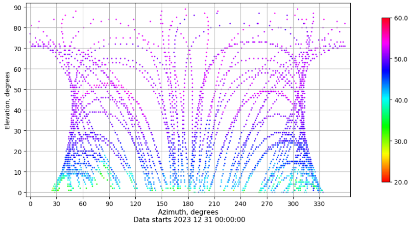
Azimuth-elevation plot for station SALA. Signal to Noise S1C Data file SALA00ESP_R_2023365.xtr
