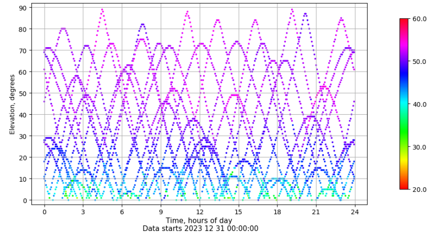
Time-elevation plot for station SALA. Signal to Noise S1C Data file SALA00ESP_R_2023365.xtr
