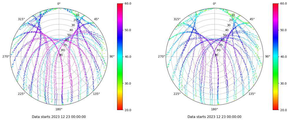
Skyplot for station SALA. Signal to Noise S1C Data file SALA00ESP_R_2023357.xtr Skyplot for station SALA. Signal to Noise S2P Data file SALA00ESP_R_2023357.xtr
