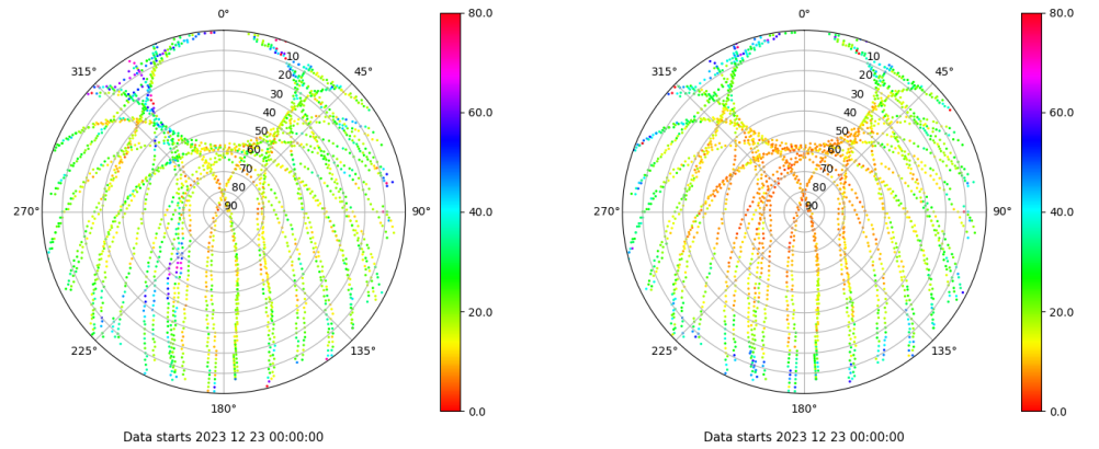
Skyplot for station SALA. Parameter M1C Data file SALA00ESP_R_2023357.xtr Skyplot for station SALA. Parameter M2P Data file SALA00ESP_R_2023357.xtr
