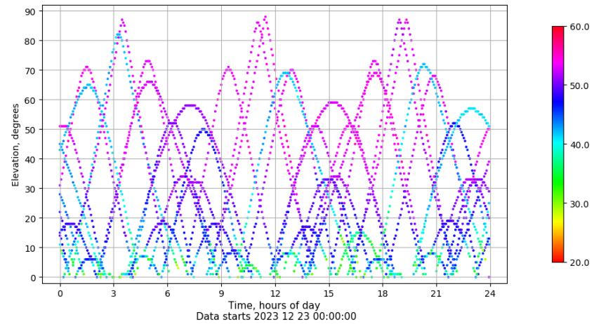
Time-elevation plot for station SALA. Signal to Noise S1C Data file SALA00ESP_R_2023357.xtr
