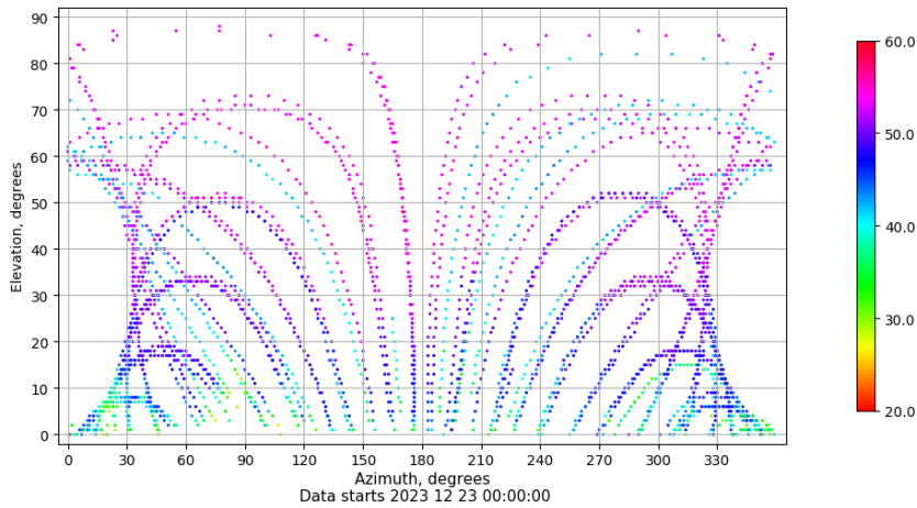
Azimuth-elevation plot for station SALA. Signal to Noise S1C Data file SALA00ESP_R_2023357.xtr
