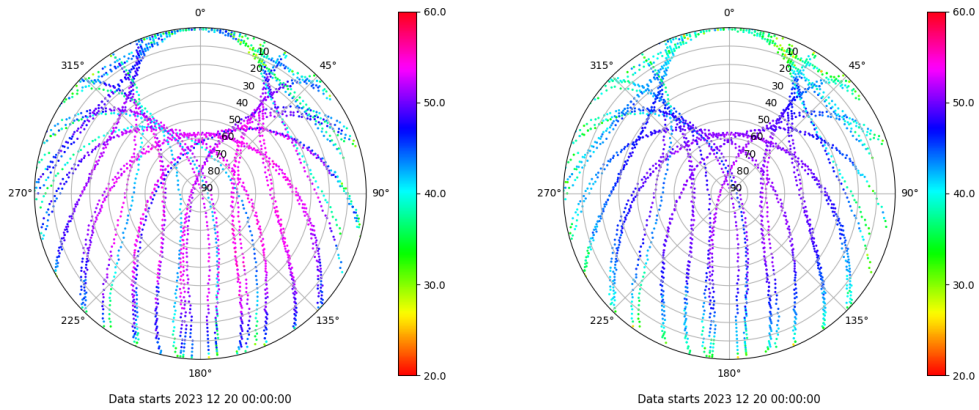
Skyplot for station SALA. Signal to Noise S1C Data file SALA00ESP_R_2023354.xtr Skyplot for station SALA. Signal to Noise S2P Data file SALA00ESP_R_2023354.xtr
