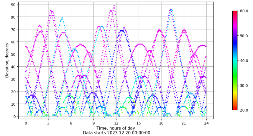
Time-elevation plot for station SALA. Signal to Noise S1C Data file SALA00ESP_R_2023354.xtr
