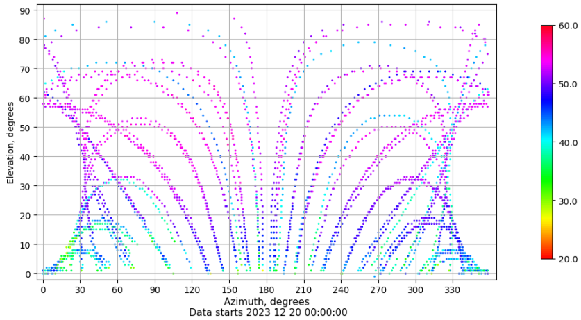
Azimuth-elevation plot for station SALA. Signal to Noise S1C Data file SALA00ESP_R_2023354.xtr
