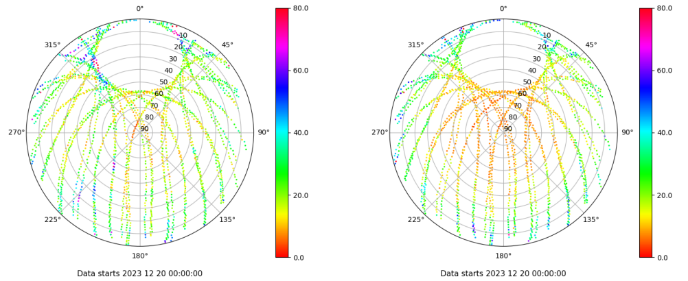
Skyplot for station SALA. Parameter M1C Data file SALA00ESP_R_2023354.xtr Skyplot for station SALA. Parameter M2P Data file SALA00ESP_R_2023354.xtr
