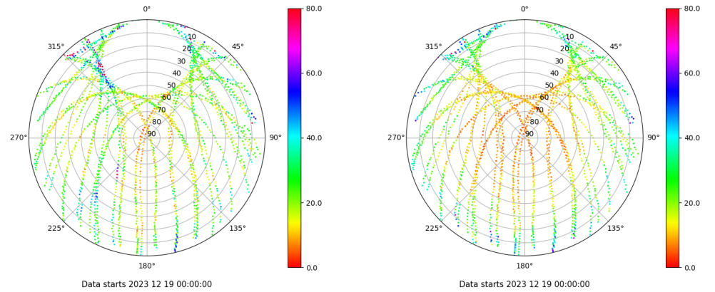
Skyplot for station SALA. Parameter M1C Data file SALA00ESP_R_2023353.xtr Skyplot for station SALA. Parameter M2P Data file SALA00ESP_R_2023353.xtr
