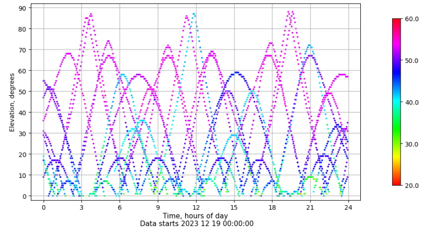
Time-elevation plot for station SALA. Signal to Noise S1C Data file SALA00ESP_R_2023353.xtr
