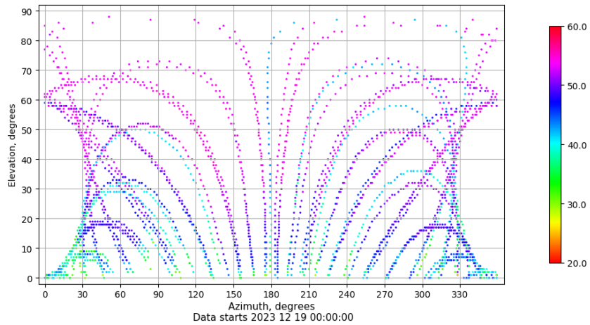
Azimuth-elevation plot for station SALA. Signal to Noise S1C Data file SALA00ESP_R_2023353.xtr
