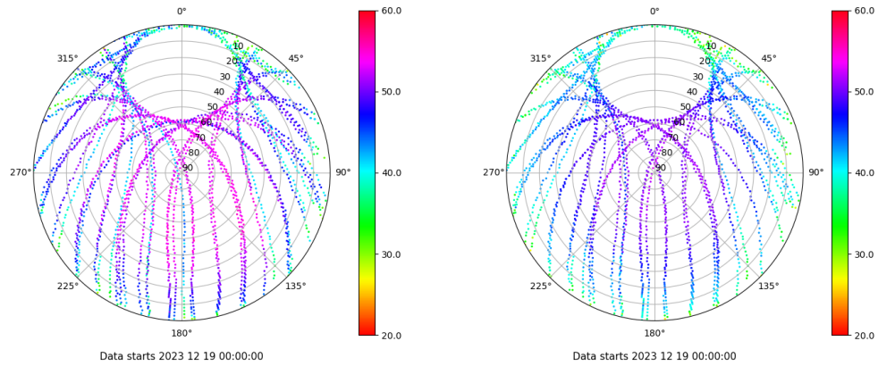
Skyplot for station SALA. Signal to Noise S1C Data file SALA00ESP_R_2023353.xtr Skyplot for station SALA. Signal to Noise S2P Data file SALA00ESP_R_2023353.xtr
