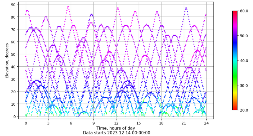
Time-elevation plot for station SALA. Signal to Noise S1C Data file SALA00ESP_R_2023348.xtr
