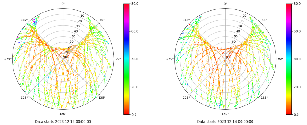
Skyplot for station SALA. Parameter M1C Data file SALA00ESP_R_2023348.xtr Skyplot for station SALA. Parameter M2S Data file SALA00ESP_R_2023348.xtr
