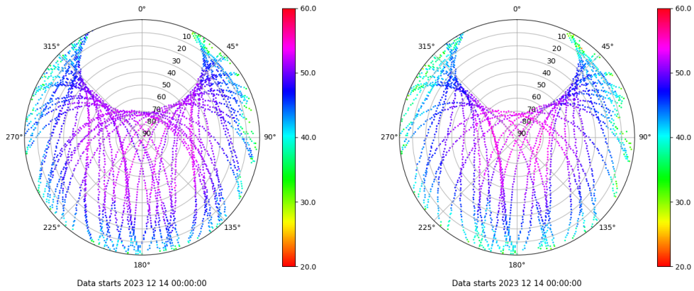
Skyplot for station SALA. Signal to Noise S1C Data file SALA00ESP_R_2023348.xtr Skyplot for station SALA. Signal to Noise S2S Data file SALA00ESP_R_2023348.xtr
