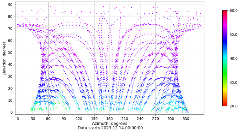
Azimuth-elevation plot for station SALA. Signal to Noise S1C Data file SALA00ESP_R_2023348.xtr
