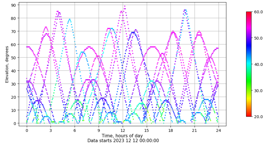
Time-elevation plot for station SALA. Signal to Noise S1C Data file SALA00ESP_R_2023346.xtr
