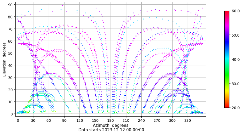
Azimuth-elevation plot for station SALA. Signal to Noise S1C Data file SALA00ESP_R_2023346.xtr
