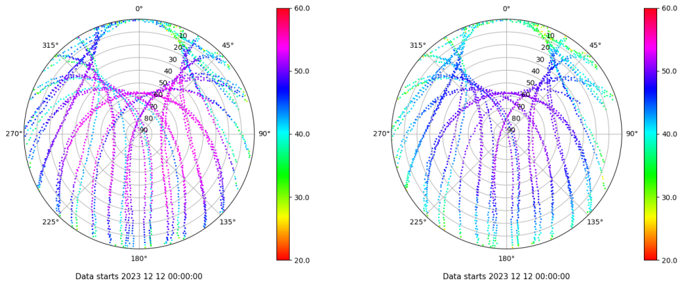
Skyplot for station SALA. Signal to Noise S1C Data file SALA00ESP_R_2023346.xtr Skyplot for station SALA. Signal to Noise S2P Data file SALA00ESP_R_2023346.xtr
