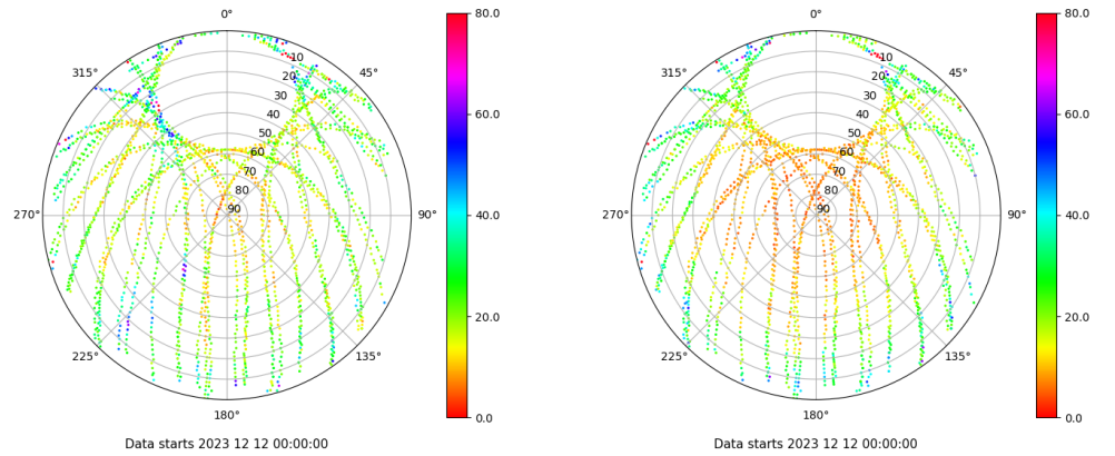
Skyplot for station SALA. Parameter M1C Data file SALA00ESP_R_2023346.xtr Skyplot for station SALA. Parameter M2P Data file SALA00ESP_R_2023346.xtr
