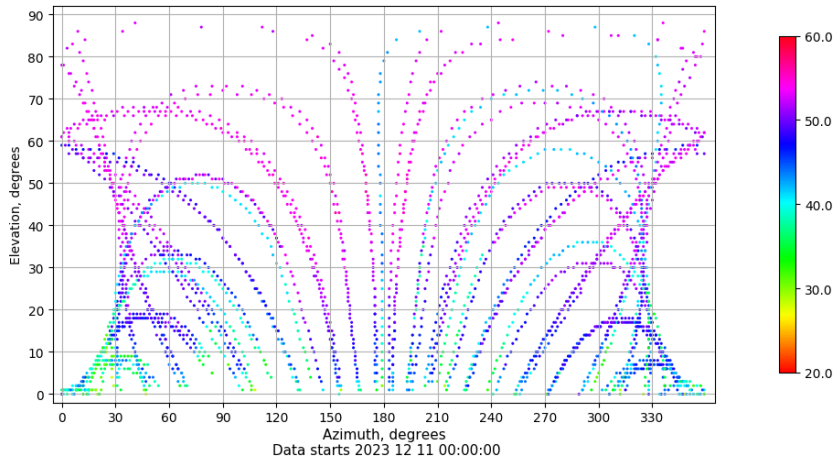
Azimuth-elevation plot for station SALA. Signal to Noise S1C Data file SALA00ESP_R_2023345.xtr
