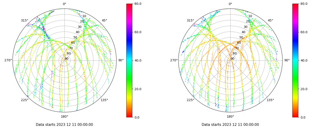
Skyplot for station SALA. Parameter M1C Data file SALA00ESP_R_2023345.xtr Skyplot for station SALA. Parameter M2P Data file SALA00ESP_R_2023345.xtr
