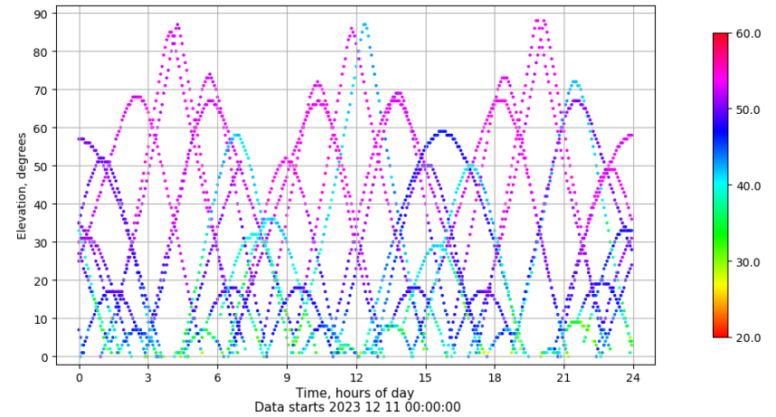
Time-elevation plot for station SALA. Signal to Noise S1C Data file SALA00ESP_R_2023345.xtr
