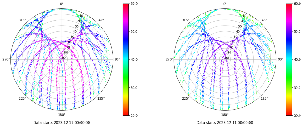
Skyplot for station SALA. Signal to Noise S1C Data file SALA00ESP_R_2023345.xtr Skyplot for station SALA. Signal to Noise S2P Data file SALA00ESP_R_2023345.xtr
