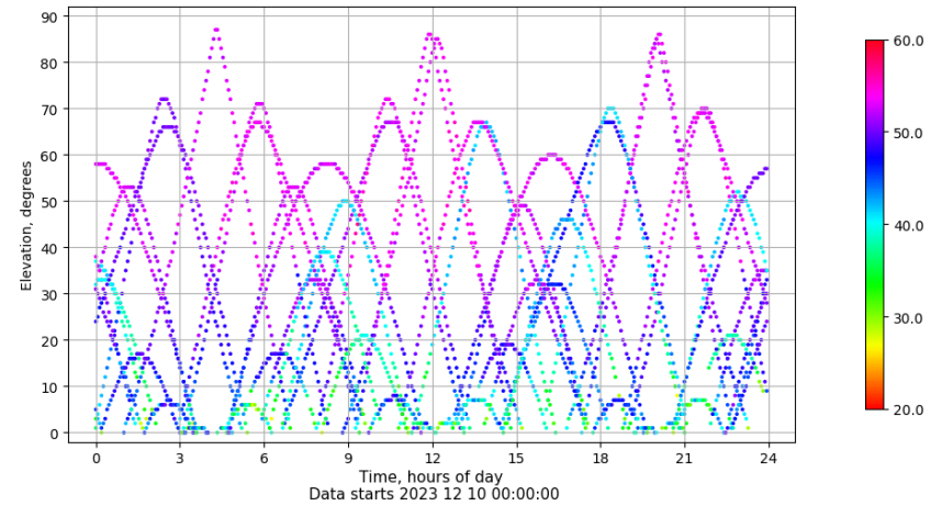
Time-elevation plot for station SALA. Signal to Noise S1C Data file SALA00ESP_R_2023344.xtr
