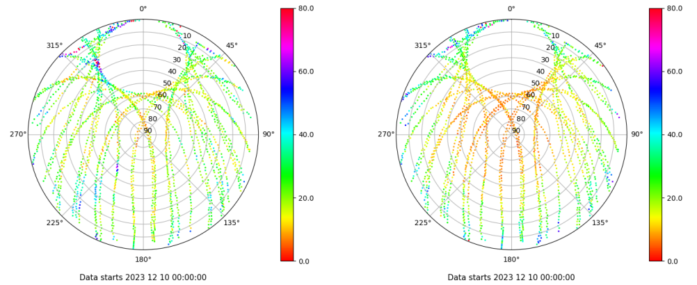
Skyplot for station SALA. Parameter M1C Data file SALA00ESP_R_2023344.xtr Skyplot for station SALA. Parameter M2P Data file SALA00ESP_R_2023344.xtr
