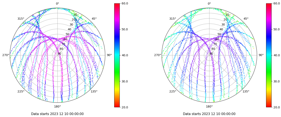
Skyplot for station SALA. Signal to Noise S1C Data file SALA00ESP_R_2023344.xtr Skyplot for station SALA. Signal to Noise S2P Data file SALA00ESP_R_2023344.xtr
