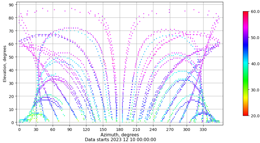
Azimuth-elevation plot for station SALA. Signal to Noise S1C Data file SALA00ESP_R_2023344.xtr
