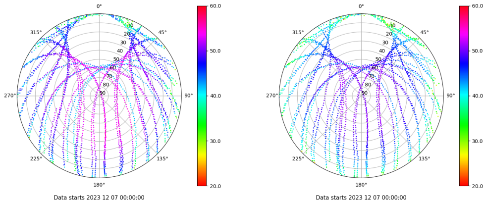
Skyplot for station SALA. Signal to Noise S1C Data file SALA00ESP_R_2023341.xtr Skyplot for station SALA. Signal to Noise S2P Data file SALA00ESP_R_2023341.xtr
