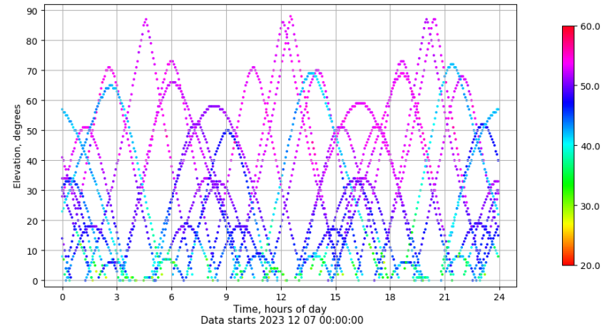
Time-elevation plot for station SALA. Signal to Noise S1C Data file SALA00ESP_R_2023341.xtr
