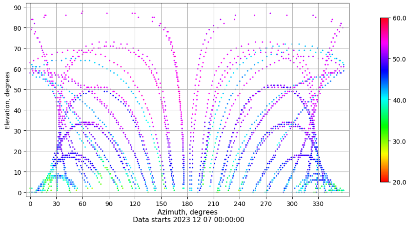
Azimuth-elevation plot for station SALA. Signal to Noise S1C Data file SALA00ESP_R_2023341.xtr
