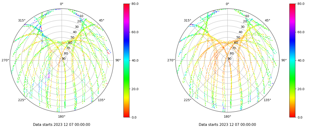
Skyplot for station SALA. Parameter M1C Data file SALA00ESP_R_2023341.xtr Skyplot for station SALA. Parameter M2P Data file SALA00ESP_R_2023341.xtr
