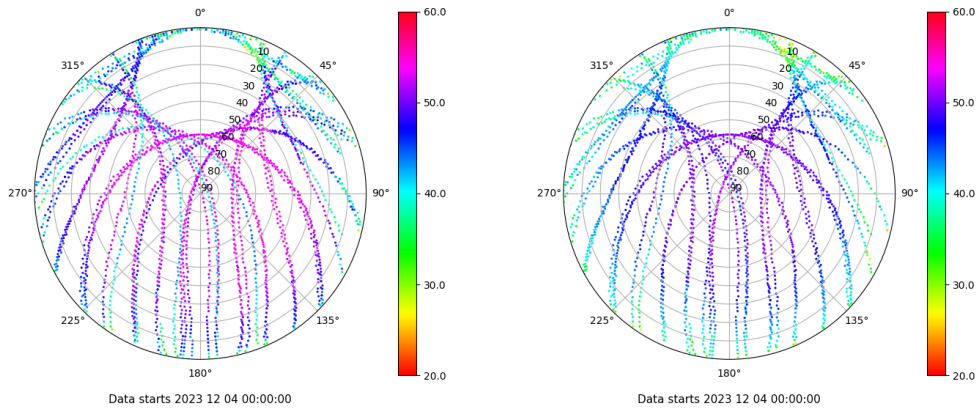
Skyplot for station SALA. Signal to Noise S1C Data file SALA00ESP_R_2023338.xtr Skyplot for station SALA. Signal to Noise S2P Data file SALA00ESP_R_2023338.xtr
