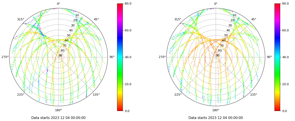
Skyplot for station SALA. Parameter M1C Data file SALA00ESP_R_2023338.xtr Skyplot for station SALA. Parameter M2P Data file SALA00ESP_R_2023338.xtr
