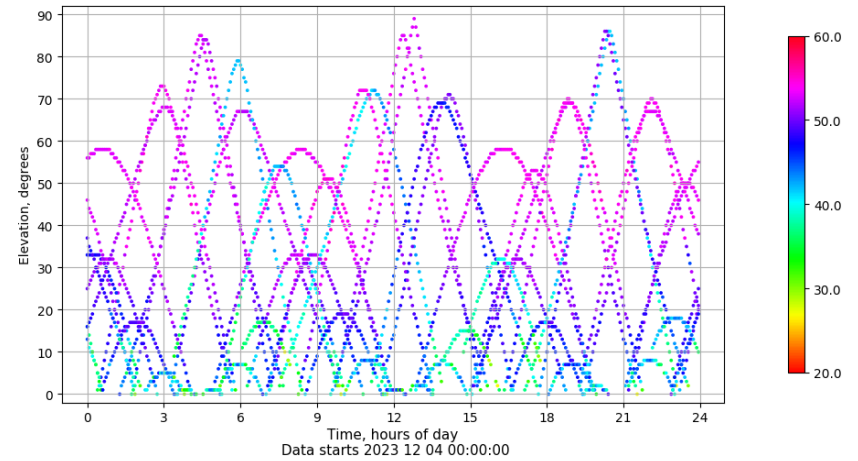
Time-elevation plot for station SALA. Signal to Noise S1C Data file SALA00ESP_R_2023338.xtr
