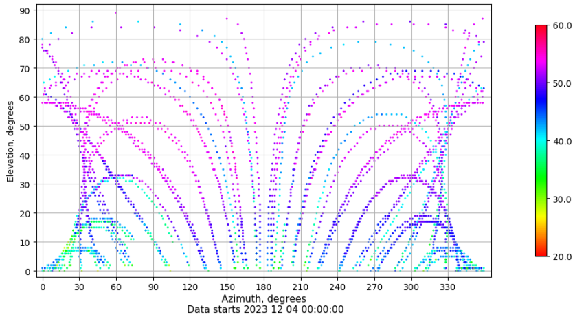
Azimuth-elevation plot for station SALA. Signal to Noise S1C Data file SALA00ESP_R_2023338.xtr
