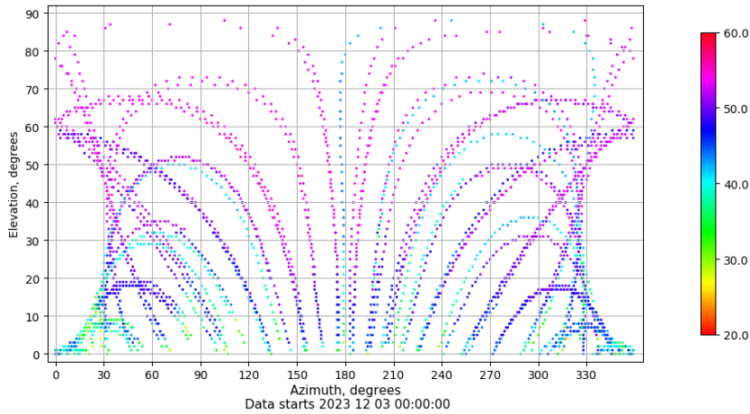
Azimuth-elevation plot for station SALA. Signal to Noise S1C Data file SALA00ESP_R_2023337.xtr
