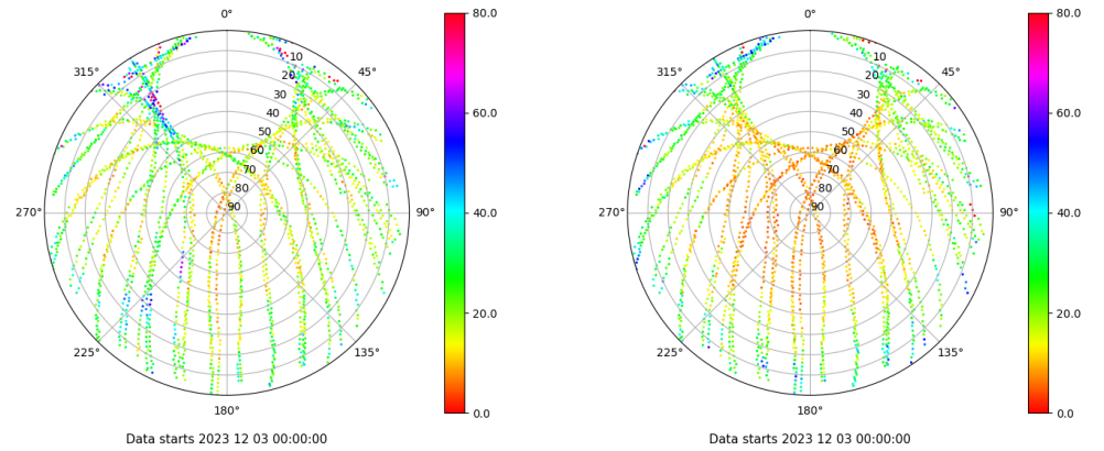
Skyplot for station SALA. Parameter M1C Data file SALA00ESP_R_2023337.xtr Skyplot for station SALA. Parameter M2P Data file SALA00ESP_R_2023337.xtr
