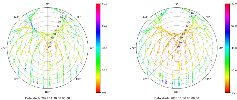
Skyplot for station SALA. Parameter M1C Data file SALA00ESP_R_2023334.xtr Skyplot for station SALA. Parameter M2P Data file SALA00ESP_R_2023334.xtr
