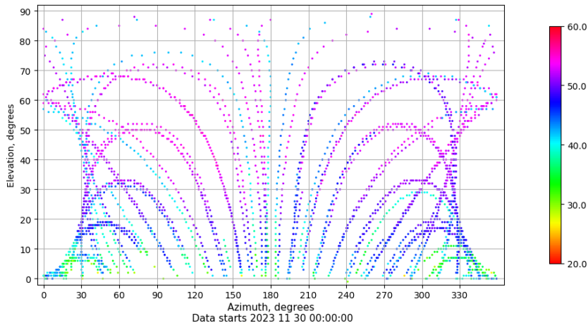
Azimuth-elevation plot for station SALA. Signal to Noise S1C Data file SALA00ESP_R_2023334.xtr
