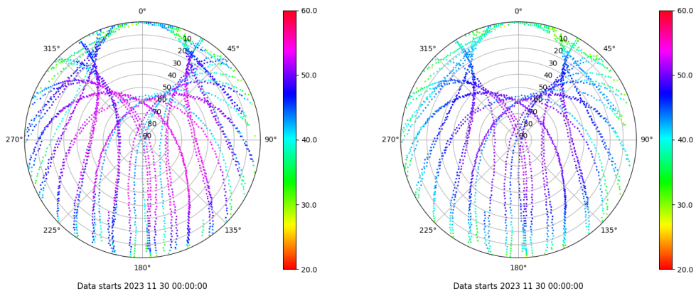
Skyplot for station SALA. Signal to Noise S1C Data file SALA00ESP_R_2023334.xtr Skyplot for station SALA. Signal to Noise S2P Data file SALA00ESP_R_2023334.xtr
