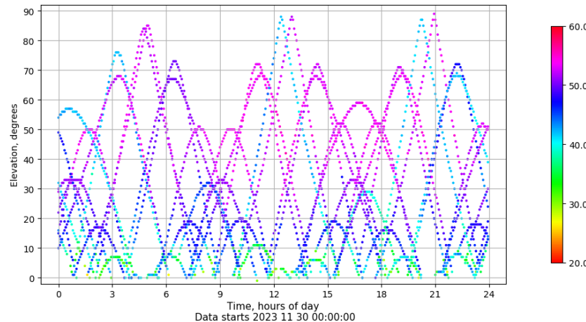
Time-elevation plot for station SALA. Signal to Noise S1C Data file SALA00ESP_R_2023334.xtr
