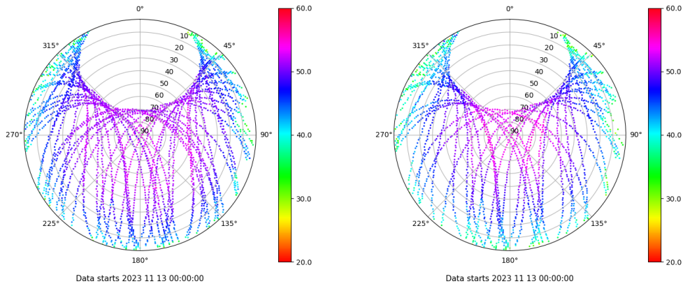
Skyplot for station SALA. Signal to Noise S1C Data file SALA00ESP_R_2023317.xtr Skyplot for station SALA. Signal to Noise S2S Data file SALA00ESP_R_2023317.xtr
