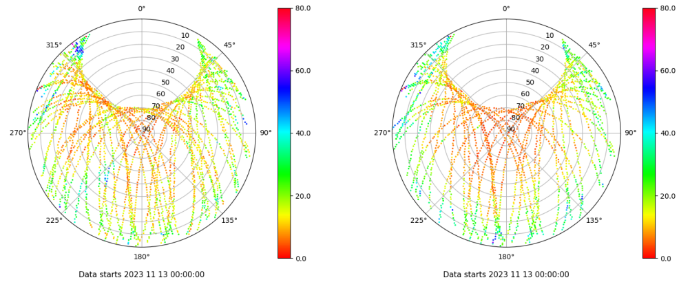
Skyplot for station SALA. Parameter M1C Data file SALA00ESP_R_2023317.xtr Skyplot for station SALA. Parameter M2S Data file SALA00ESP_R_2023317.xtr
