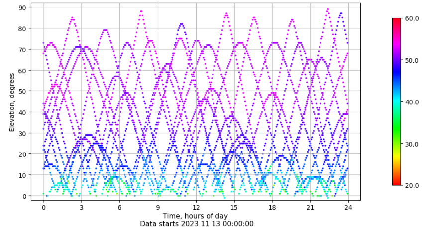
Time-elevation plot for station SALA. Signal to Noise S1C Data file SALA00ESP_R_2023317.xtr
