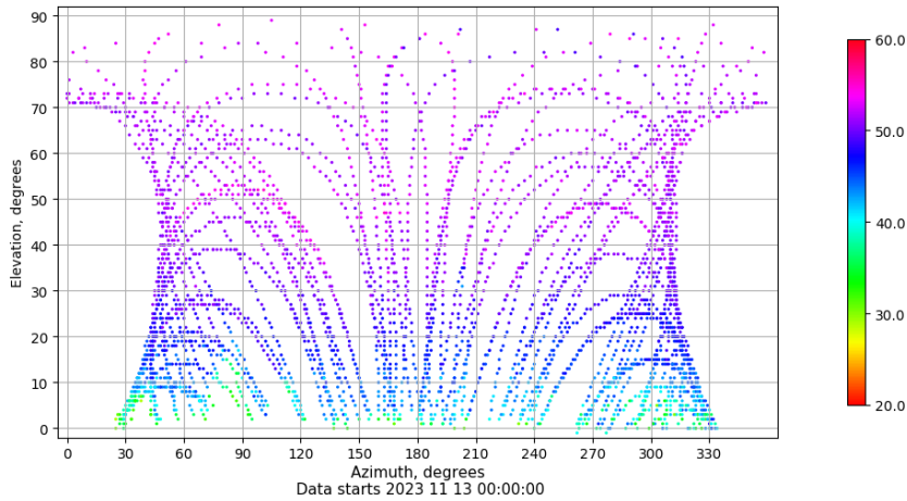
Azimuth-elevation plot for station SALA. Signal to Noise S1C Data file SALA00ESP_R_2023317.xtr
