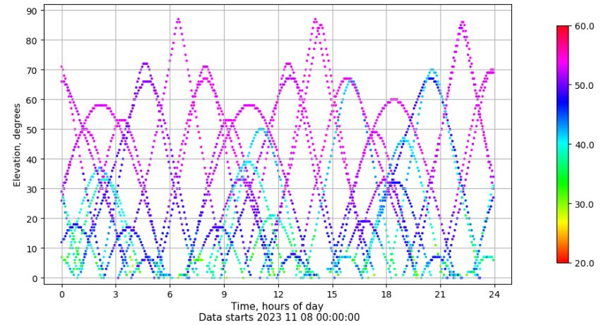
Time-elevation plot for station SALA. Signal to Noise S1C Data file SALA00ESP_R_2023312.xtr
