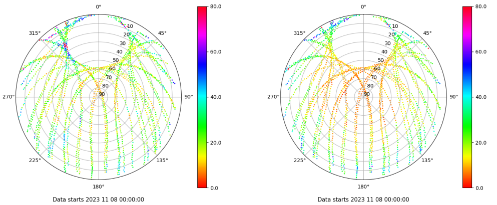
Skyplot for station SALA. Parameter M1C Data file SALA00ESP_R_2023312.xtr Skyplot for station SALA. Parameter M2P Data file SALA00ESP_R_2023312.xtr
