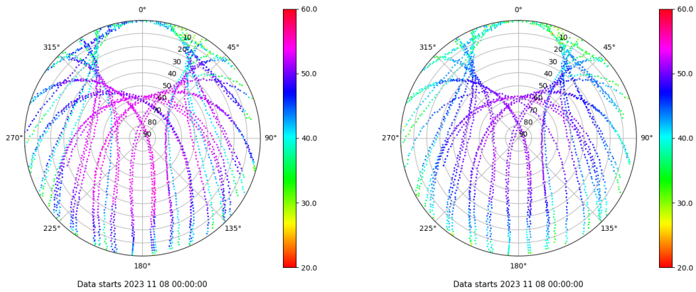
Skyplot for station SALA. Signal to Noise S1C Data file SALA00ESP_R_2023312.xtr Skyplot for station SALA. Signal to Noise S2P Data file SALA00ESP_R_2023312.xtr
