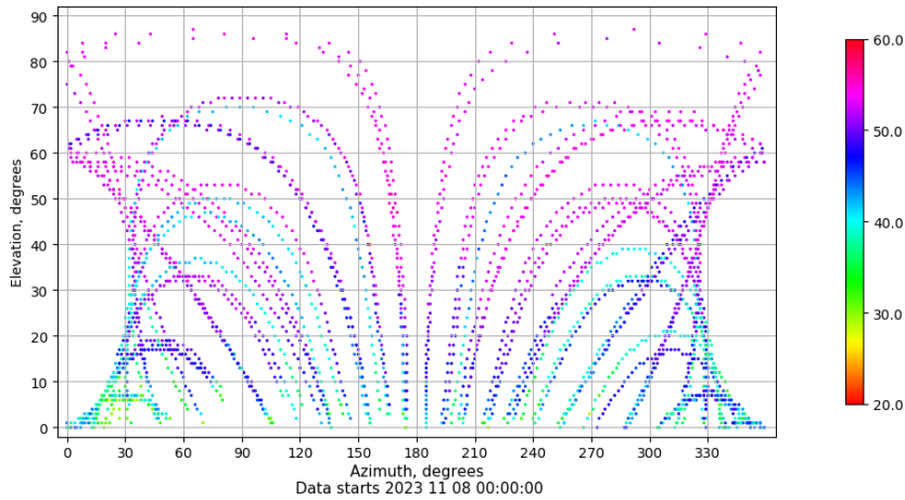
Azimuth-elevation plot for station SALA. Signal to Noise S1C Data file SALA00ESP_R_2023312.xtr
