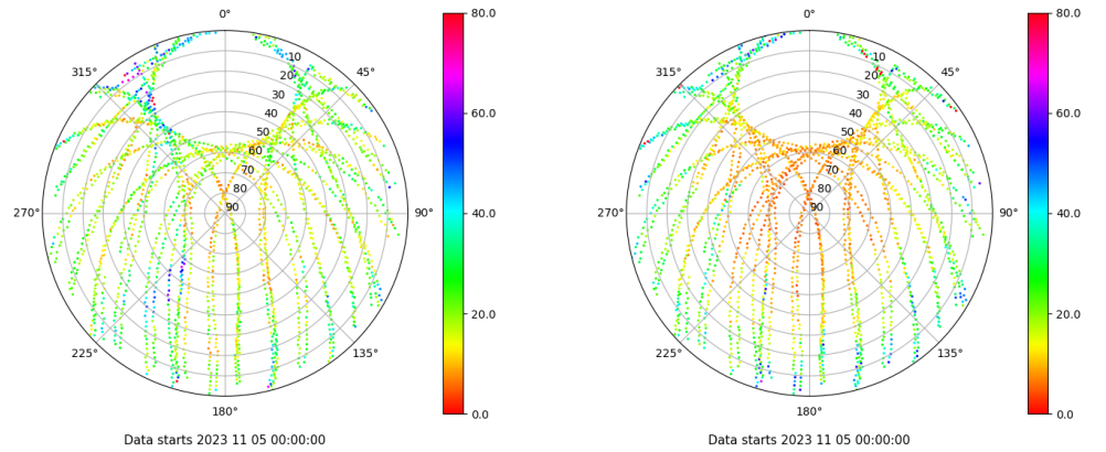
Skyplot for station SALA. Parameter M1C Data file SALA00ESP_R_2023309.xtr Skyplot for station SALA. Parameter M2P Data file SALA00ESP_R_2023309.xtr
