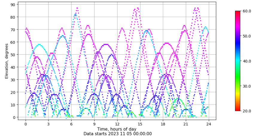
Time-elevation plot for station SALA. Signal to Noise S1C Data file SALA00ESP_R_2023309.xtr
