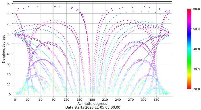
Azimuth-elevation plot for station SALA. Signal to Noise S1C Data file SALA00ESP_R_2023309.xtr
