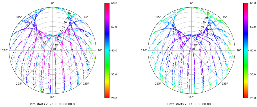
Skyplot for station SALA. Signal to Noise S1C Data file SALA00ESP_R_2023309.xtr Skyplot for station SALA. Signal to Noise S2P Data file SALA00ESP_R_2023309.xtr
