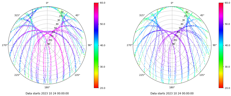
Skyplot for station SALA. Signal to Noise S1C Data file SALA00ESP_R_2023297.xtr Skyplot for station SALA. Signal to Noise S2P Data file SALA00ESP_R_2023297.xtr
