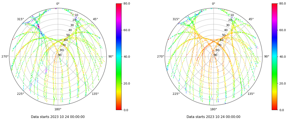
Skyplot for station SALA. Parameter M1C Data file SALA00ESP_R_2023297.xtr Skyplot for station SALA. Parameter M2P Data file SALA00ESP_R_2023297.xtr
