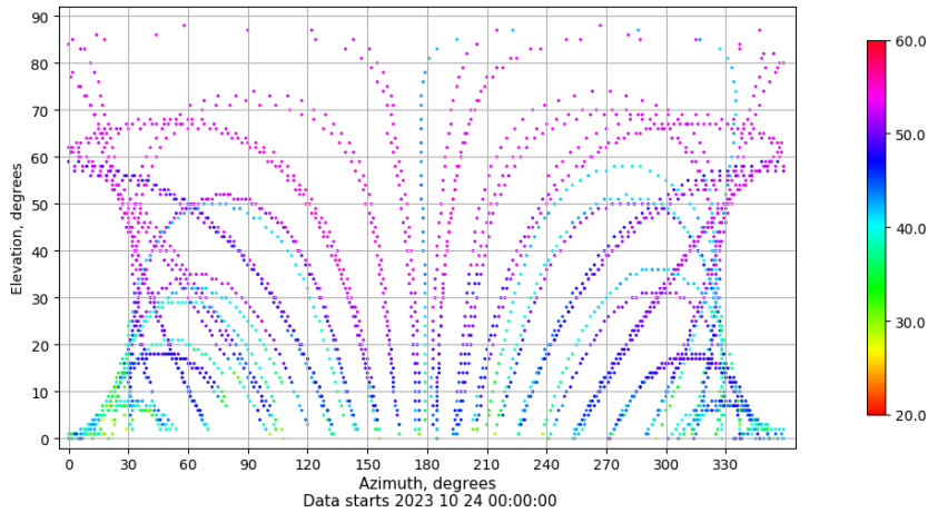
Azimuth-elevation plot for station SALA. Signal to Noise S1C Data file SALA00ESP_R_2023297.xtr
