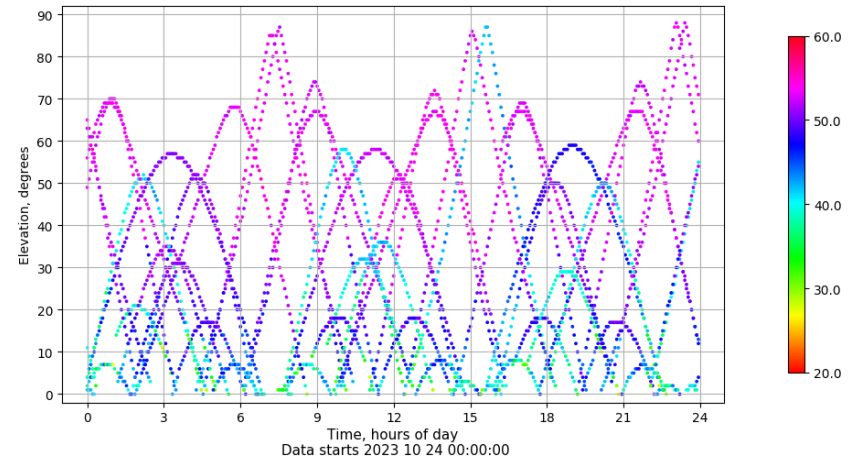
Time-elevation plot for station SALA. Signal to Noise S1C Data file SALA00ESP_R_2023297.xtr
