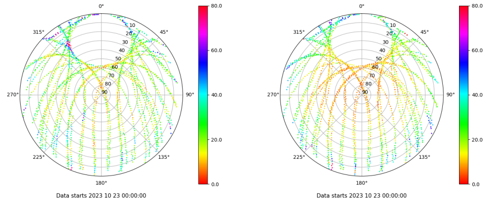
Skyplot for station SALA. Parameter M1C Data file SALA00ESP_R_2023296.xtr Skyplot for station SALA. Parameter M2P Data file SALA00ESP_R_2023296.xtr
