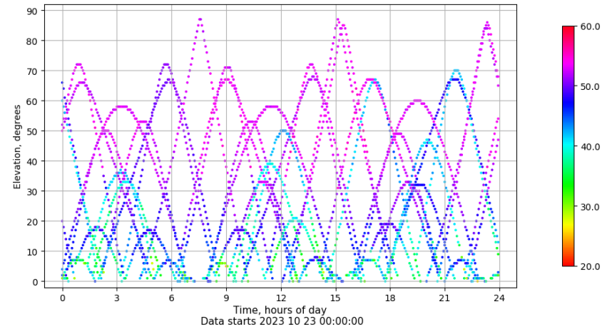
Time-elevation plot for station SALA. Signal to Noise S1C Data file SALA00ESP_R_2023296.xtr
