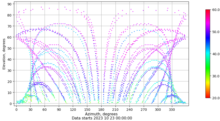
Azimuth-elevation plot for station SALA. Signal to Noise S1C Data file SALA00ESP_R_2023296.xtr
