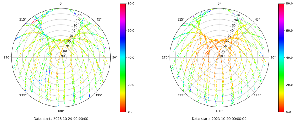
Skyplot for station SALA. Parameter M1C Data file SALA00ESP_R_2023293.xtr Skyplot for station SALA. Parameter M2P Data file SALA00ESP_R_2023293.xtr
