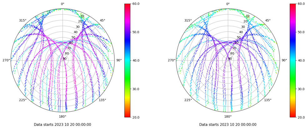
Skyplot for station SALA. Signal to Noise S1C Data file SALA00ESP_R_2023293.xtr Skyplot for station SALA. Signal to Noise S2P Data file SALA00ESP_R_2023293.xtr
