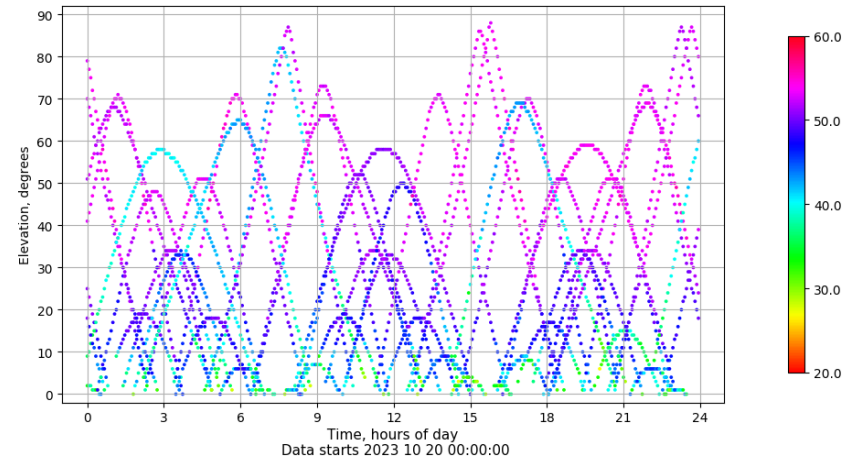
Time-elevation plot for station SALA. Signal to Noise S1C Data file SALA00ESP_R_2023293.xtr
