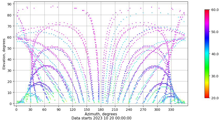
Azimuth-elevation plot for station SALA. Signal to Noise S1C Data file SALA00ESP_R_2023293.xtr
