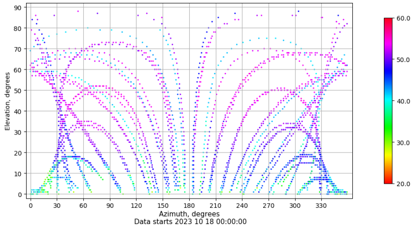
Azimuth-elevation plot for station SALA. Signal to Noise S1C Data file SALA00ESP_R_2023291.xtr
