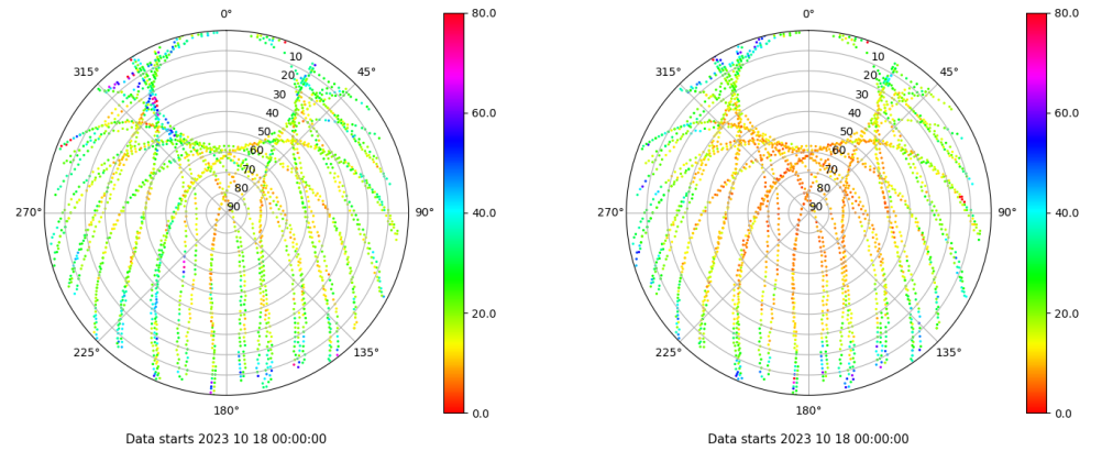
Skyplot for station SALA. Parameter M1C Data file SALA00ESP_R_2023291.xtr Skyplot for station SALA. Parameter M2P Data file SALA00ESP_R_2023291.xtr
