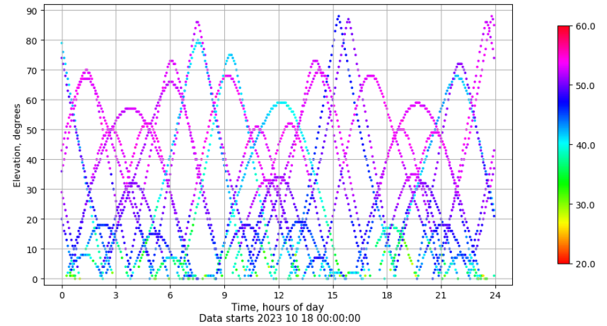
Time-elevation plot for station SALA. Signal to Noise S1C Data file SALA00ESP_R_2023291.xtr
