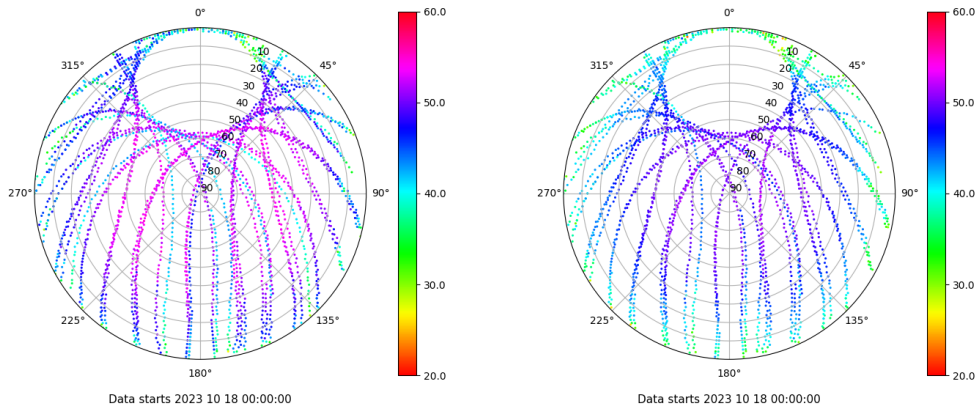
Skyplot for station SALA. Signal to Noise S1C Data file SALA00ESP_R_2023291.xtr Skyplot for station SALA. Signal to Noise S2P Data file SALA00ESP_R_2023291.xtr
