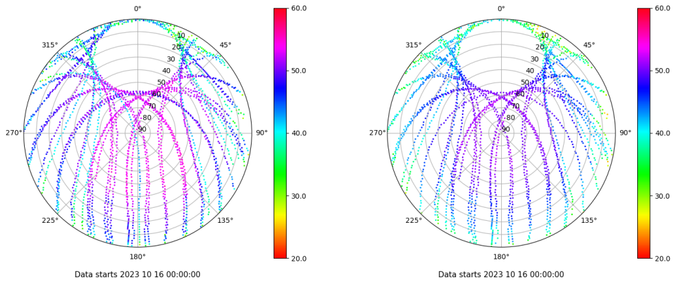
Skyplot for station SALA. Signal to Noise S1C Data file SALA00ESP_R_2023289.xtr Skyplot for station SALA. Signal to Noise S2P Data file SALA00ESP_R_2023289.xtr
