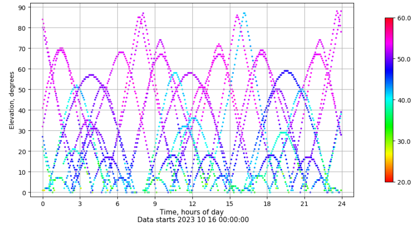
Time-elevation plot for station SALA. Signal to Noise S1C Data file SALA00ESP_R_2023289.xtr
