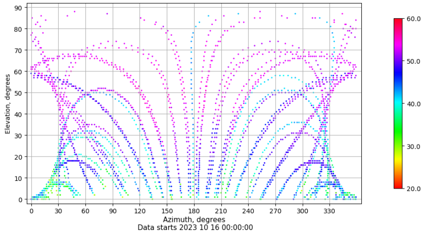
Azimuth-elevation plot for station SALA. Signal to Noise S1C Data file SALA00ESP_R_2023289.xtr
