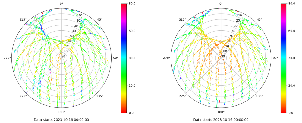
Skyplot for station SALA. Parameter M1C Data file SALA00ESP_R_2023289.xtr Skyplot for station SALA. Parameter M2P Data file SALA00ESP_R_2023289.xtr
