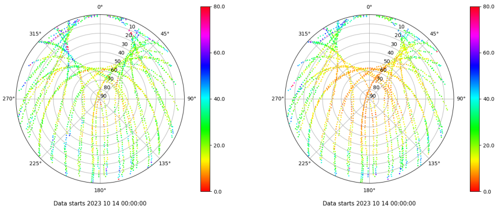
Skyplot for station SALA. Parameter M1C Data file SALA00ESP_R_2023287.xtr Skyplot for station SALA. Parameter M2P Data file SALA00ESP_R_2023287.xtr
