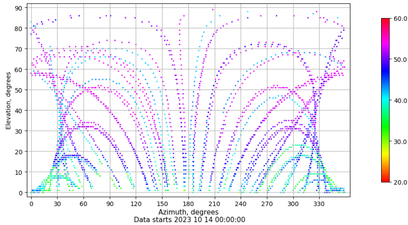
Azimuth-elevation plot for station SALA. Signal to Noise S1C Data file SALA00ESP_R_2023287.xtr
