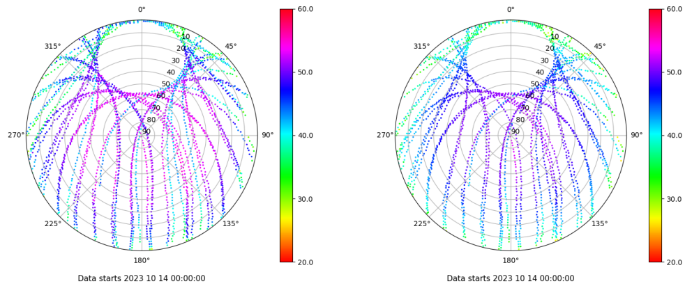
Skyplot for station SALA. Signal to Noise S1C Data file SALA00ESP_R_2023287.xtr Skyplot for station SALA. Signal to Noise S2P Data file SALA00ESP_R_2023287.xtr
