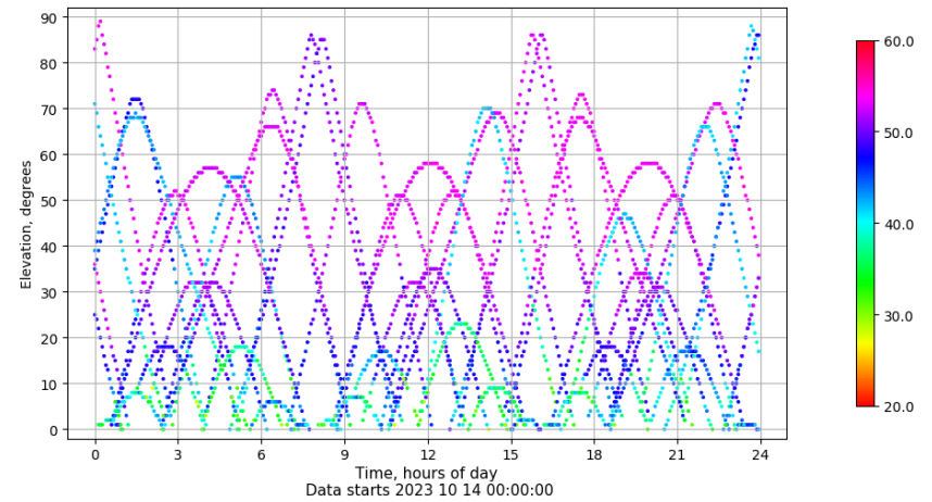
Time-elevation plot for station SALA. Signal to Noise S1C Data file SALA00ESP_R_2023287.xtr
