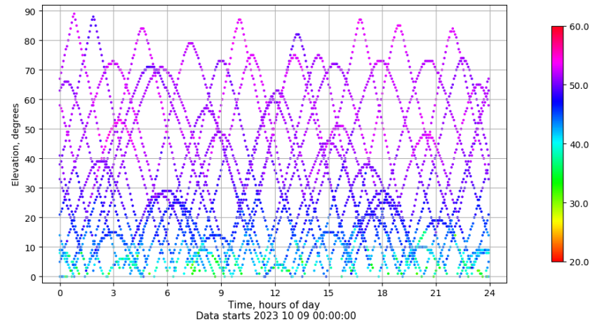
Time-elevation plot for station SALA. Signal to Noise S1C Data file SALA00ESP_R_2023282.xtr
