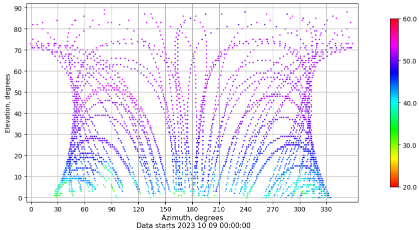
Azimuth-elevation plot for station SALA. Signal to Noise S1C Data file SALA00ESP_R_2023282.xtr
