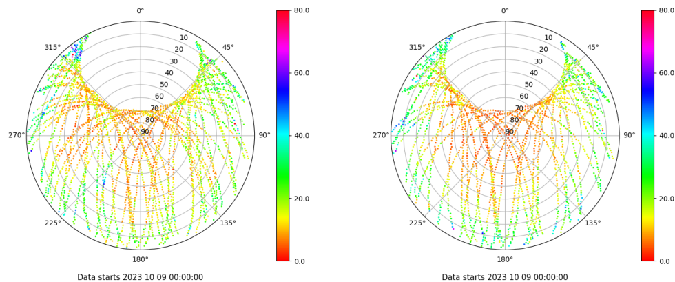
Skyplot for station SALA. Parameter M1C Data file SALA00ESP_R_2023282.xtr Skyplot for station SALA. Parameter M2S Data file SALA00ESP_R_2023282.xtr
