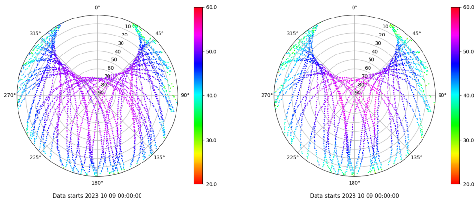
Skyplot for station SALA. Signal to Noise S1C Data file SALA00ESP_R_2023282.xtr Skyplot for station SALA. Signal to Noise S2S Data file SALA00ESP_R_2023282.xtr
