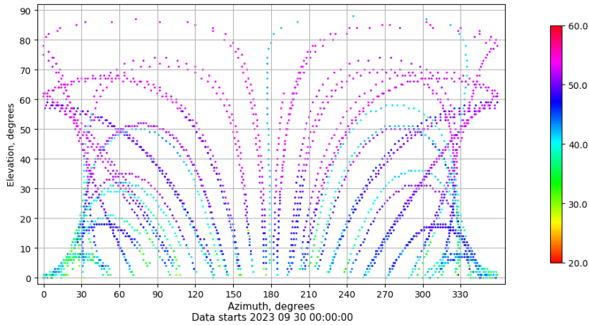
Azimuth-elevation plot for station SALA. Signal to Noise S1C Data file SALA00ESP_R_2023273.xtr
