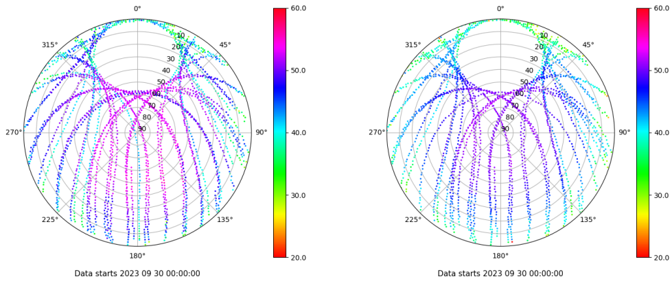
Skyplot for station SALA. Signal to Noise S1C Data file SALA00ESP_R_2023273.xtr Skyplot for station SALA. Signal to Noise S2P Data file SALA00ESP_R_2023273.xtr
