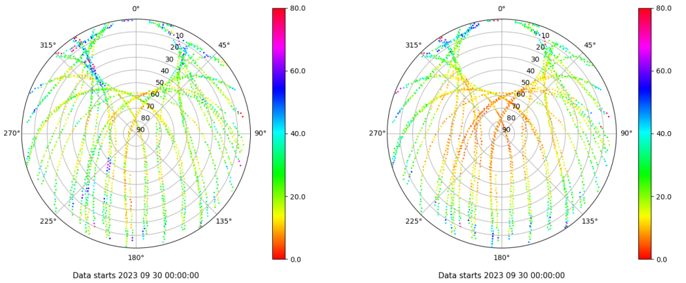
Skyplot for station SALA. Parameter M1C Data file SALA00ESP_R_2023273.xtr Skyplot for station SALA. Parameter M2P Data file SALA00ESP_R_2023273.xtr
