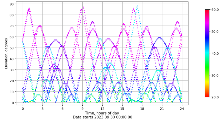
Time-elevation plot for station SALA. Signal to Noise S1C Data file SALA00ESP_R_2023273.xtr
