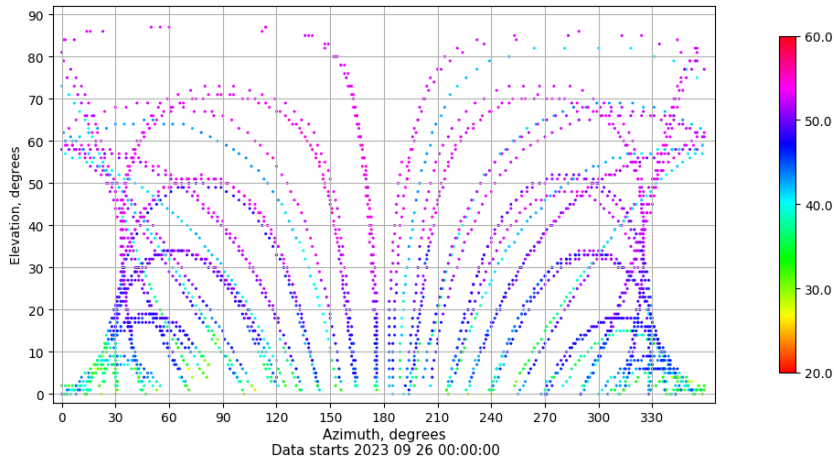
Azimuth-elevation plot for station SALA. Signal to Noise S1C Data file SALA00ESP_R_2023269.xtr
