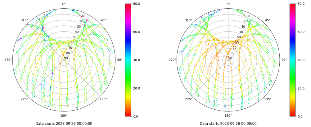
Skyplot for station SALA. Parameter M1C Data file SALA00ESP_R_2023269.xtr Skyplot for station SALA. Parameter M2P Data file SALA00ESP_R_2023269.xtr
