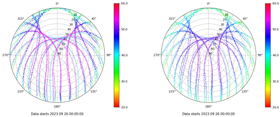
Skyplot for station SALA. Signal to Noise S1C Data file SALA00ESP_R_2023269.xtr Skyplot for station SALA. Signal to Noise S2P Data file SALA00ESP_R_2023269.xtr
