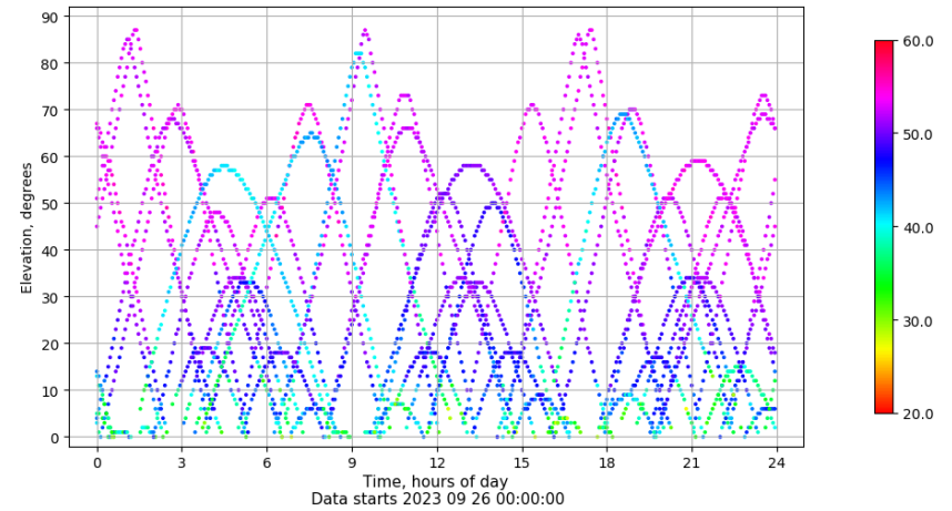
Time-elevation plot for station SALA. Signal to Noise S1C Data file SALA00ESP_R_2023269.xtr
