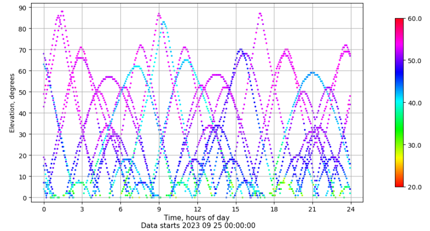
Time-elevation plot for station SALA. Signal to Noise S1C Data file SALA00ESP_R_2023268.xtr
