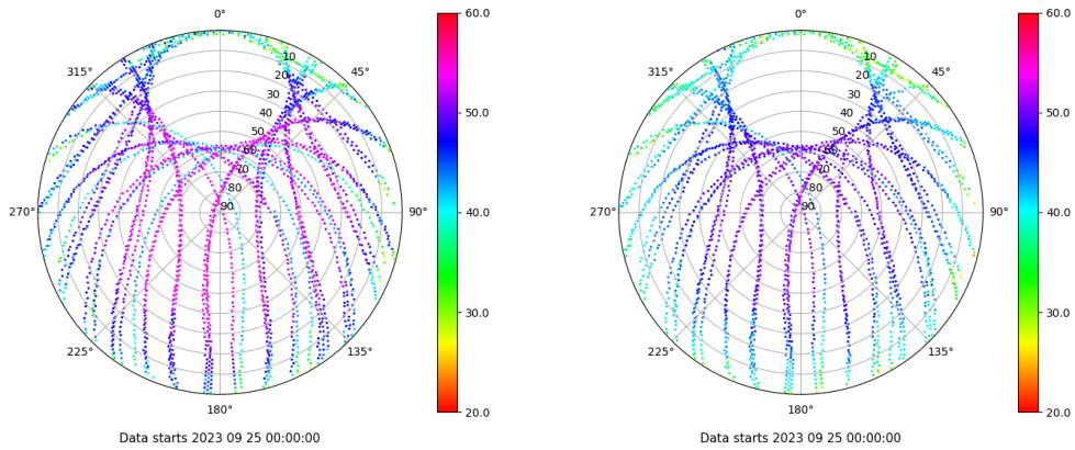
Skyplot for station SALA. Signal to Noise S1C Data file SALA00ESP_R_2023268.xtr Skyplot for station SALA. Signal to Noise S2P Data file SALA00ESP_R_2023268.xtr
