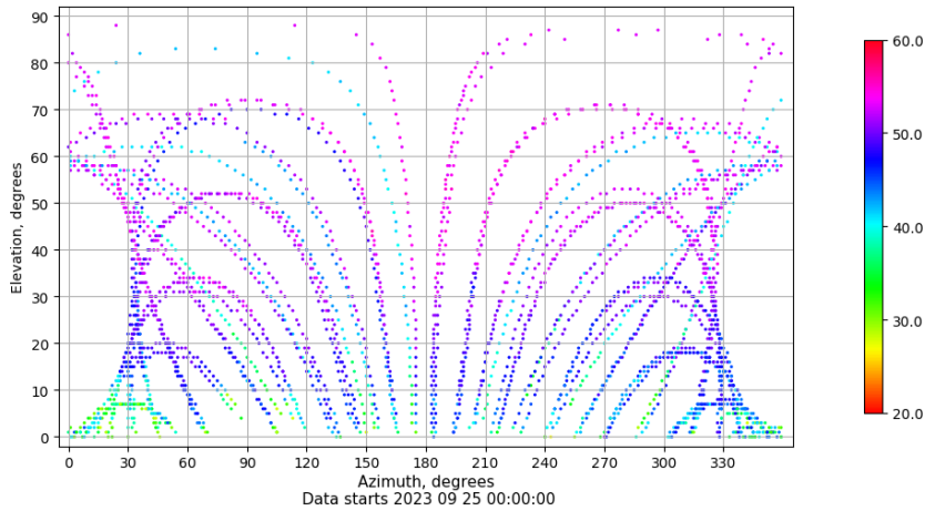
Azimuth-elevation plot for station SALA. Signal to Noise S1C Data file SALA00ESP_R_2023268.xtr
