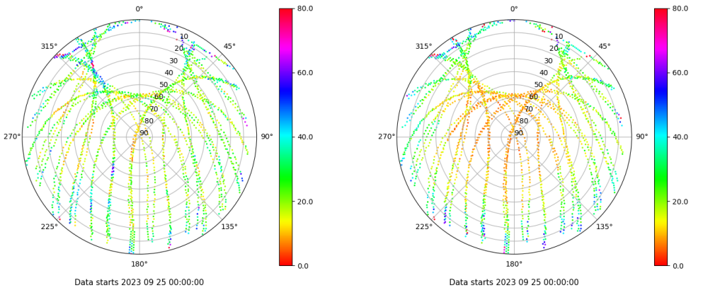
Skyplot for station SALA. Parameter M1C Data file SALA00ESP_R_2023268.xtr Skyplot for station SALA. Parameter M2P Data file SALA00ESP_R_2023268.xtr
