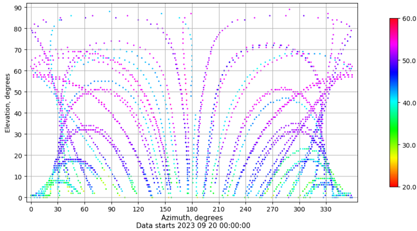
Azimuth-elevation plot for station SALA. Signal to Noise S1C Data file SALA00ESP_R_2023263.xtr
