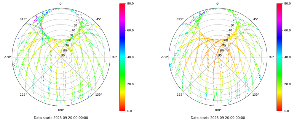
Skyplot for station SALA. Parameter M1C Data file SALA00ESP_R_2023263.xtr Skyplot for station SALA. Parameter M2P Data file SALA00ESP_R_2023263.xtr
