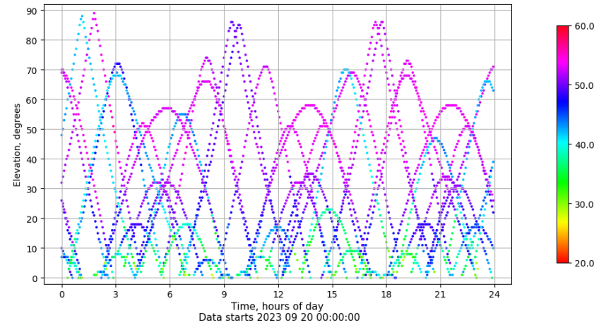
Time-elevation plot for station SALA. Signal to Noise S1C Data file SALA00ESP_R_2023263.xtr
