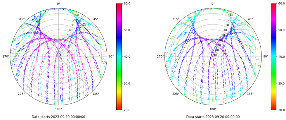
Skyplot for station SALA. Signal to Noise S1C Data file SALA00ESP_R_2023263.xtr Skyplot for station SALA. Signal to Noise S2P Data file SALA00ESP_R_2023263.xtr
