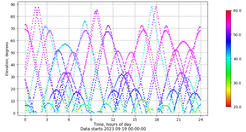
Time-elevation plot for station SALA. Signal to Noise S1C Data file SALA00ESP_R_2023262.xtr
