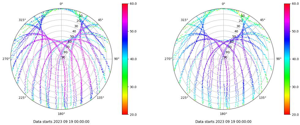
Skyplot for station SALA. Signal to Noise S1C Data file SALA00ESP_R_2023262.xtr Skyplot for station SALA. Signal to Noise S2P Data file SALA00ESP_R_2023262.xtr
