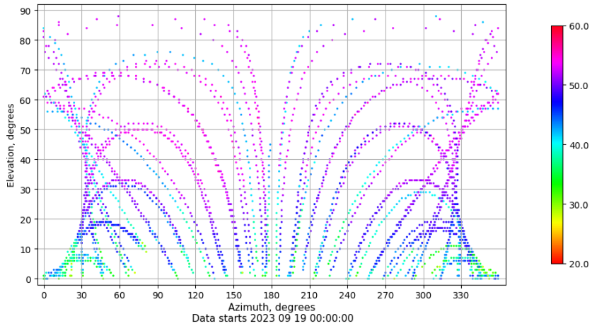
Azimuth-elevation plot for station SALA. Signal to Noise S1C Data file SALA00ESP_R_2023262.xtr
