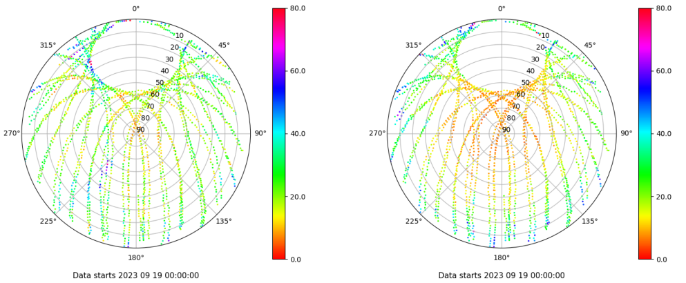
Skyplot for station SALA. Parameter M1C Data file SALA00ESP_R_2023262.xtr Skyplot for station SALA. Parameter M2P Data file SALA00ESP_R_2023262.xtr
