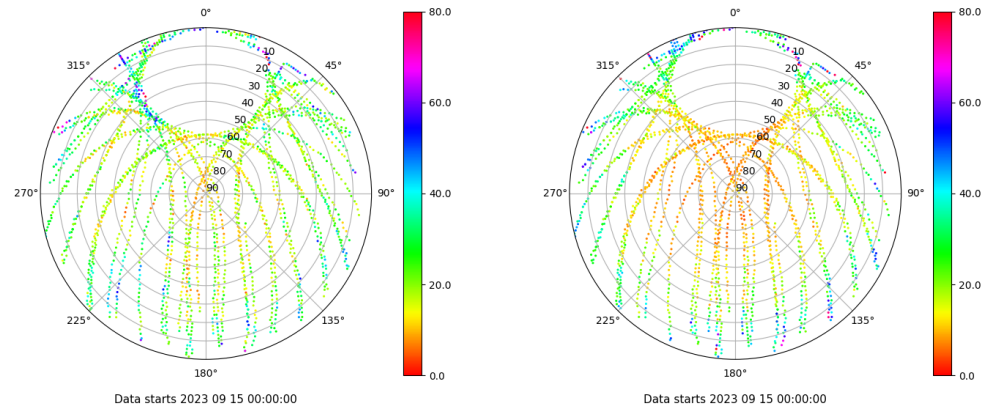
Skyplot for station SALA. Parameter M1C Data file SALA00ESP_R_2023258.xtr Skyplot for station SALA. Parameter M2P Data file SALA00ESP_R_2023258.xtr
