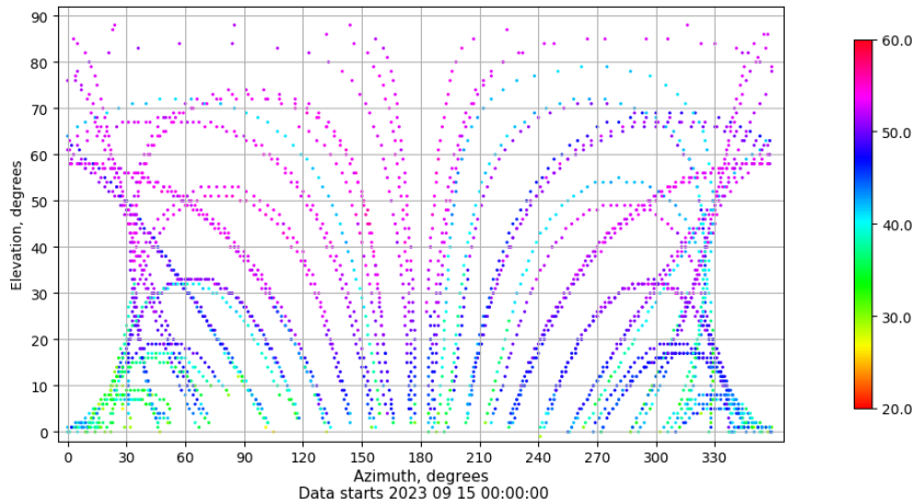
Azimuth-elevation plot for station SALA. Signal to Noise S1C Data file SALA00ESP_R_2023258.xtr
