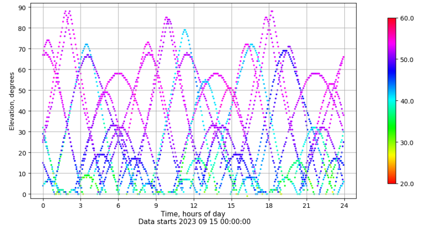
Time-elevation plot for station SALA. Signal to Noise S1C Data file SALA00ESP_R_2023258.xtr
