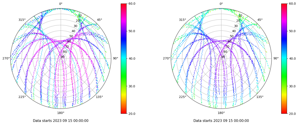
Skyplot for station SALA. Signal to Noise S1C Data file SALA00ESP_R_2023258.xtr Skyplot for station SALA. Signal to Noise S2P Data file SALA00ESP_R_2023258.xtr
