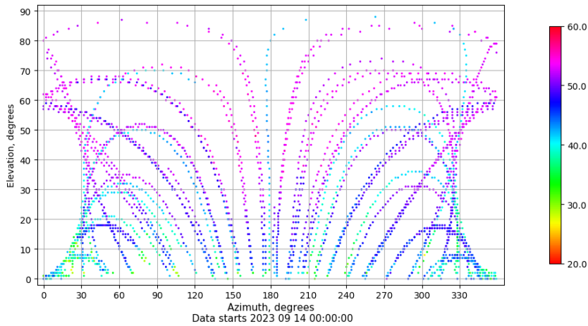
Azimuth-elevation plot for station SALA. Signal to Noise S1C Data file SALA00ESP_R_2023257.xtr
