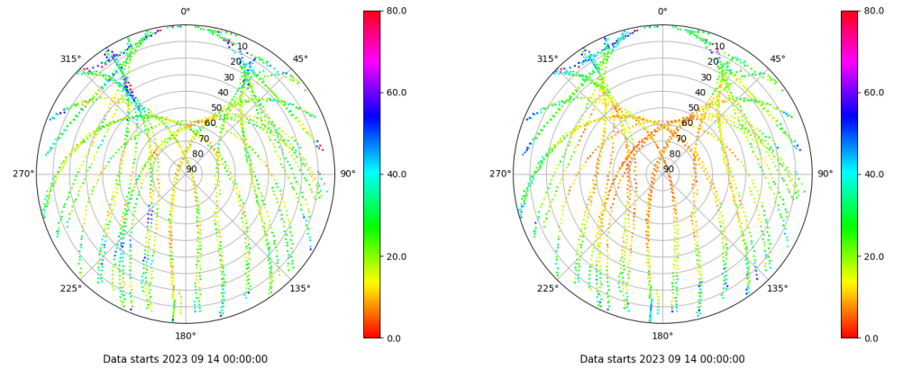
Skyplot for station SALA. Parameter M1C Data file SALA00ESP_R_2023257.xtr Skyplot for station SALA. Parameter M2P Data file SALA00ESP_R_2023257.xtr
