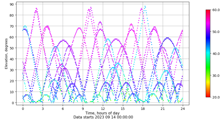
Time-elevation plot for station SALA. Signal to Noise S1C Data file SALA00ESP_R_2023257.xtr
