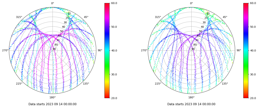
Skyplot for station SALA. Signal to Noise S1C Data file SALA00ESP_R_2023257.xtr Skyplot for station SALA. Signal to Noise S2P Data file SALA00ESP_R_2023257.xtr
