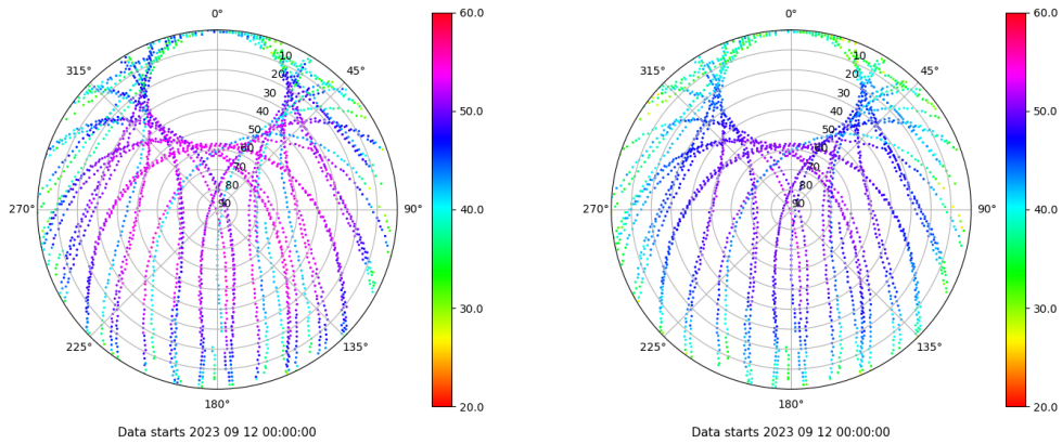
Skyplot for station SALA. Signal to Noise S1C Data file SALA00ESP_R_2023255.xtr Skyplot for station SALA. Signal to Noise S2P Data file SALA00ESP_R_2023255.xtr
