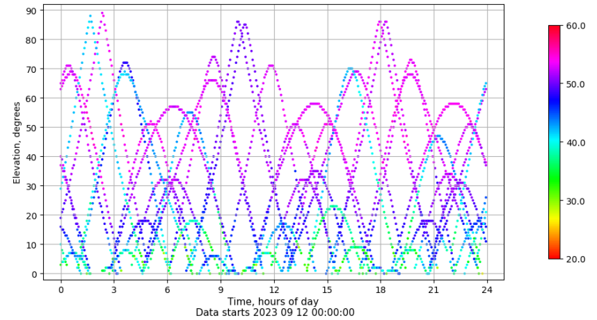
Time-elevation plot for station SALA. Signal to Noise S1C Data file SALA00ESP_R_2023255.xtr
