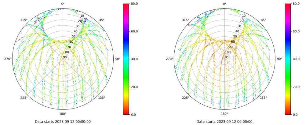
Skyplot for station SALA. Parameter M1C Data file SALA00ESP_R_2023255.xtr Skyplot for station SALA. Parameter M2P Data file SALA00ESP_R_2023255.xtr
