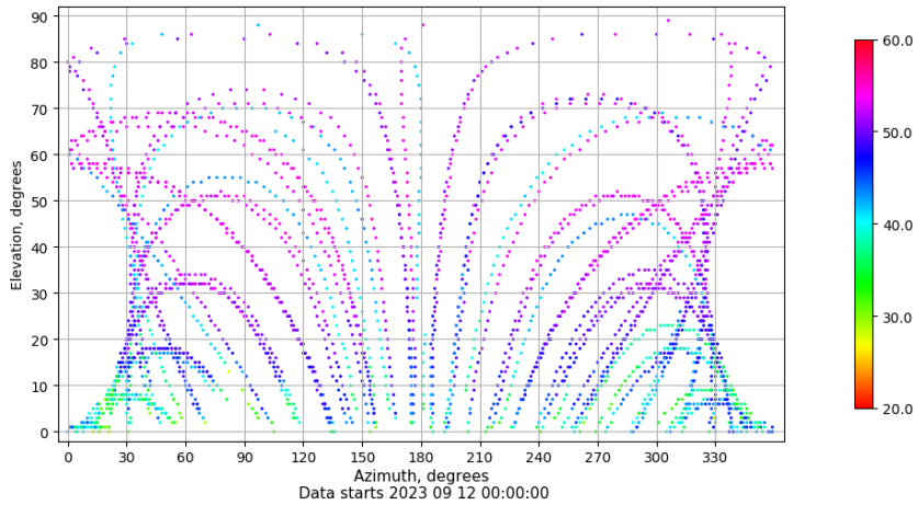
Azimuth-elevation plot for station SALA. Signal to Noise S1C Data file SALA00ESP_R_2023255.xtr
