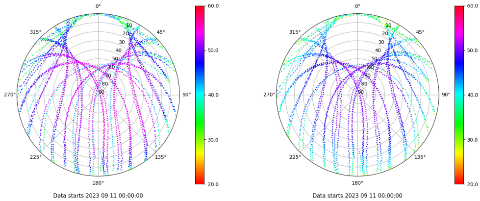
Skyplot for station SALA. Signal to Noise S1C Data file SALA00ESP_R_2023254.xtr Skyplot for station SALA. Signal to Noise S2P Data file SALA00ESP_R_2023254.xtr
