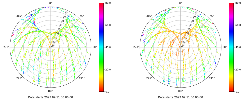
Skyplot for station SALA. Parameter M1C Data file SALA00ESP_R_2023254.xtr Skyplot for station SALA. Parameter M2P Data file SALA00ESP_R_2023254.xtr
