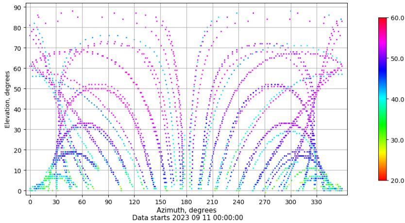
Azimuth-elevation plot for station SALA. Signal to Noise S1C Data file SALA00ESP_R_2023254.xtr
