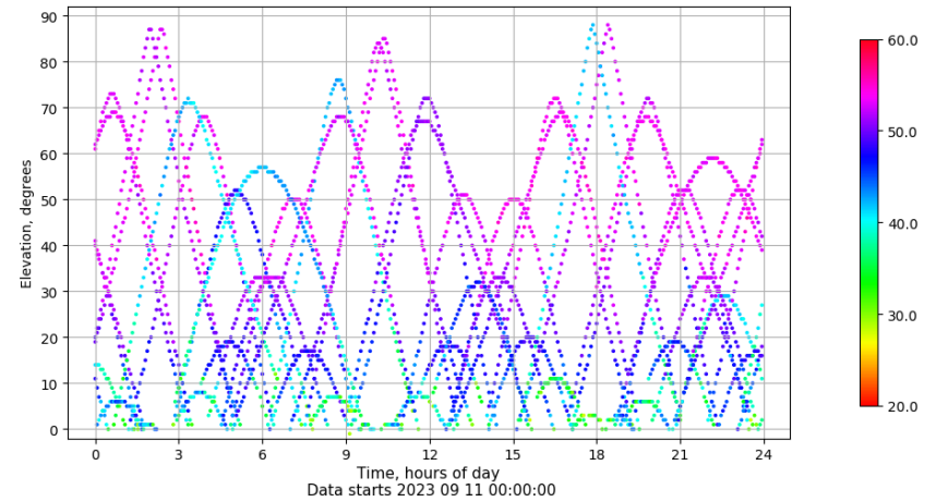
Time-elevation plot for station SALA. Signal to Noise S1C Data file SALA00ESP_R_2023254.xtr
