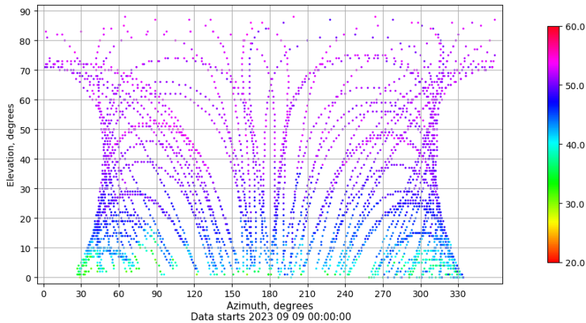
Azimuth-elevation plot for station SALA. Signal to Noise S1C Data file SALA00ESP_R_2023252.xtr
