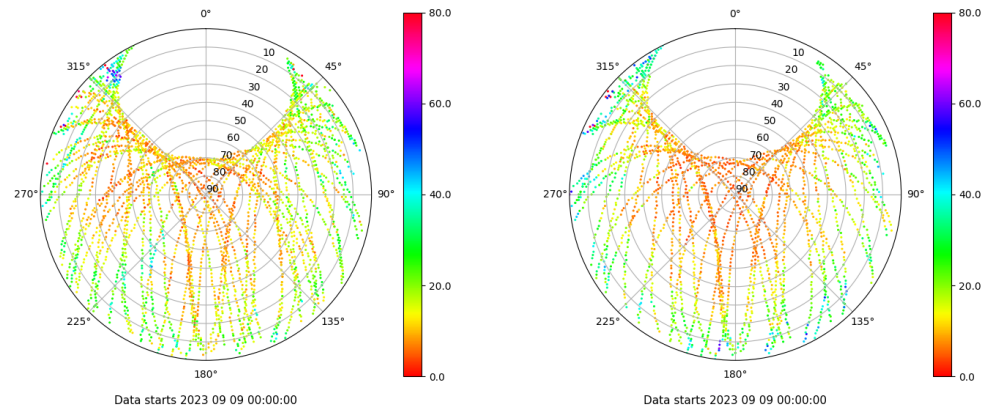
Skyplot for station SALA. Parameter M1C Data file SALA00ESP_R_2023252.xtr Skyplot for station SALA. Parameter M2S Data file SALA00ESP_R_2023252.xtr
