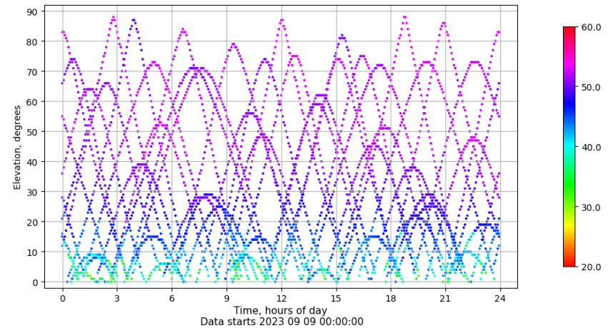
Time-elevation plot for station SALA. Signal to Noise S1C Data file SALA00ESP_R_2023252.xtr
