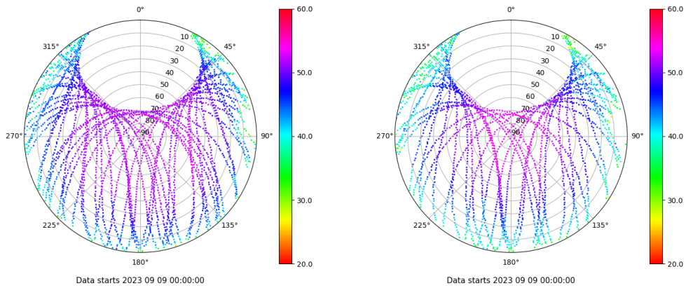
Skyplot for station SALA. Signal to Noise S1C Data file SALA00ESP_R_2023252.xtr Skyplot for station SALA. Signal to Noise S2S Data file SALA00ESP_R_2023252.xtr
