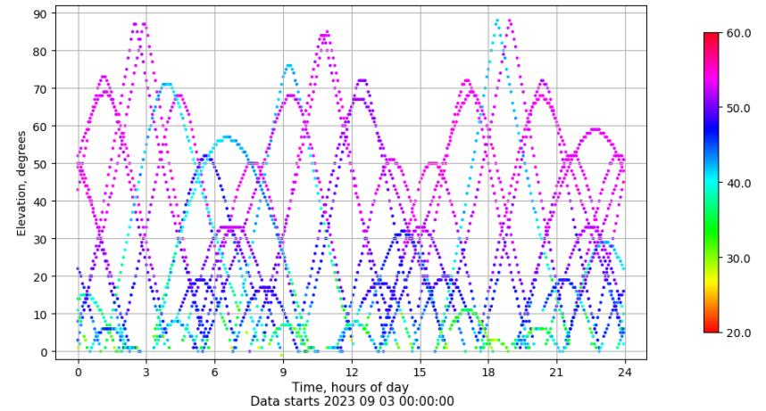
Time-elevation plot for station SALA. Signal to Noise S1C Data file SALA00ESP_R_2023246.xtr
