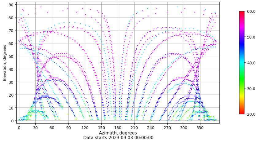
Azimuth-elevation plot for station SALA. Signal to Noise S1C Data file SALA00ESP_R_2023246.xtr
