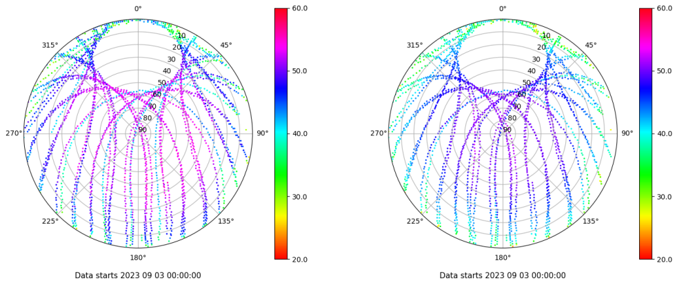
Skyplot for station SALA. Signal to Noise S1C Data file SALA00ESP_R_2023246.xtr Skyplot for station SALA. Signal to Noise S2P Data file SALA00ESP_R_2023246.xtr
