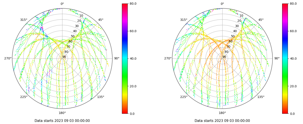
Skyplot for station SALA. Parameter M1C Data file SALA00ESP_R_2023246.xtr Skyplot for station SALA. Parameter M2P Data file SALA00ESP_R_2023246.xtr
