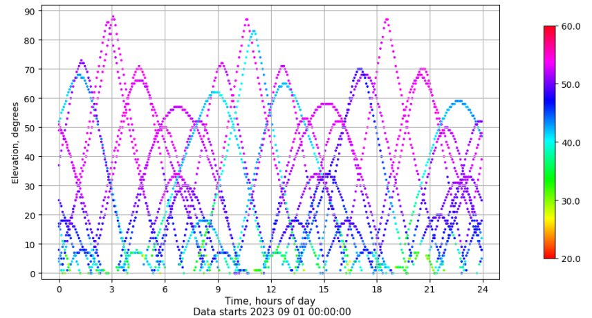
Time-elevation plot for station SALA. Signal to Noise S1C Data file SALA00ESP_R_2023244.xtr
