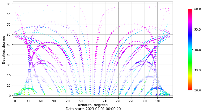
Azimuth-elevation plot for station SALA. Signal to Noise S1C Data file SALA00ESP_R_2023244.xtr
