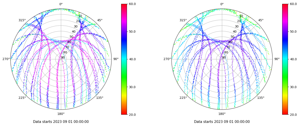
Skyplot for station SALA. Signal to Noise S1C Data file SALA00ESP_R_2023244.xtr Skyplot for station SALA. Signal to Noise S2P Data file SALA00ESP_R_2023244.xtr
