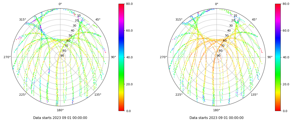
Skyplot for station SALA. Parameter M1C Data file SALA00ESP_R_2023244.xtr Skyplot for station SALA. Parameter M2P Data file SALA00ESP_R_2023244.xtr
