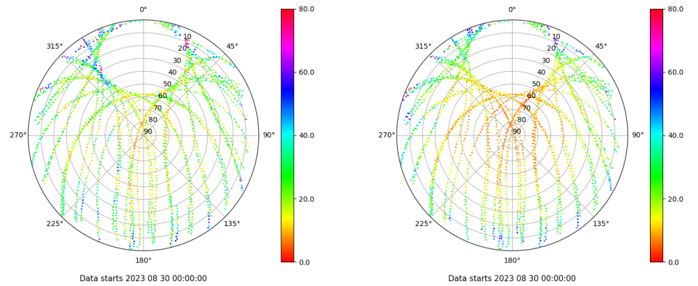
Skyplot for station SALA. Parameter M1C Data file SALA00ESP_R_2023242.xtr Skyplot for station SALA. Parameter M2P Data file SALA00ESP_R_2023242.xtr
