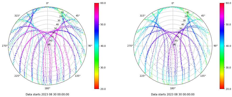
Skyplot for station SALA. Signal to Noise S1C Data file SALA00ESP_R_2023242.xtr Skyplot for station SALA. Signal to Noise S2P Data file SALA00ESP_R_2023242.xtr
