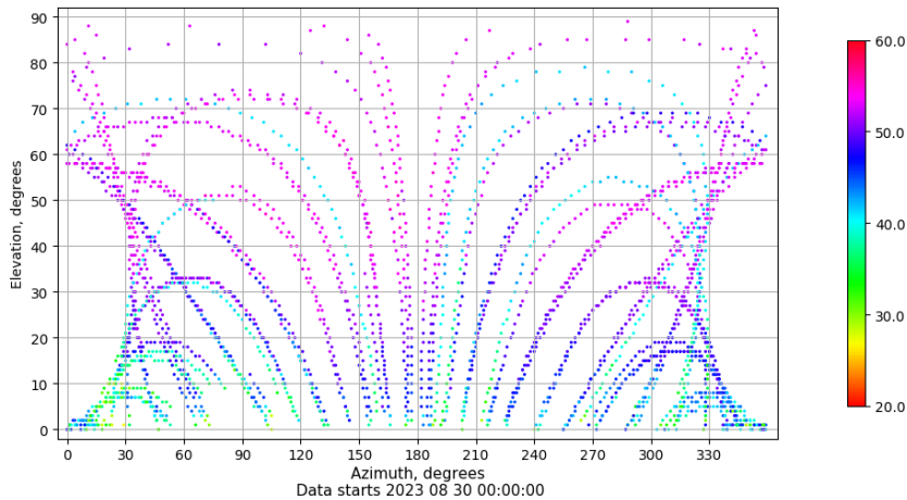
Azimuth-elevation plot for station SALA. Signal to Noise S1C Data file SALA00ESP_R_2023242.xtr
