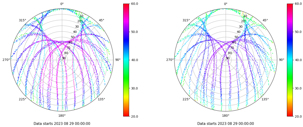
Skyplot for station SALA. Signal to Noise S1C Data file SALA00ESP_R_2023241.xtr Skyplot for station SALA. Signal to Noise S2P Data file SALA00ESP_R_2023241.xtr
