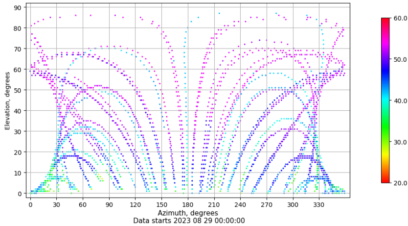
Azimuth-elevation plot for station SALA. Signal to Noise S1C Data file SALA00ESP_R_2023241.xtr
