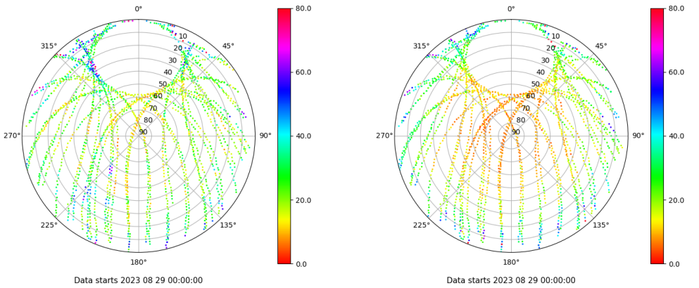
Skyplot for station SALA. Parameter M1C Data file SALA00ESP_R_2023241.xtr Skyplot for station SALA. Parameter M2P Data file SALA00ESP_R_2023241.xtr
