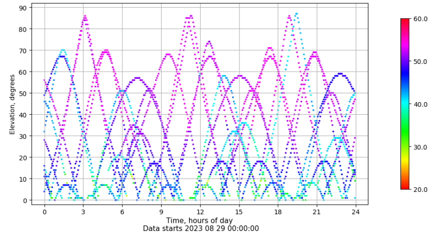
Time-elevation plot for station SALA. Signal to Noise S1C Data file SALA00ESP_R_2023241.xtr
