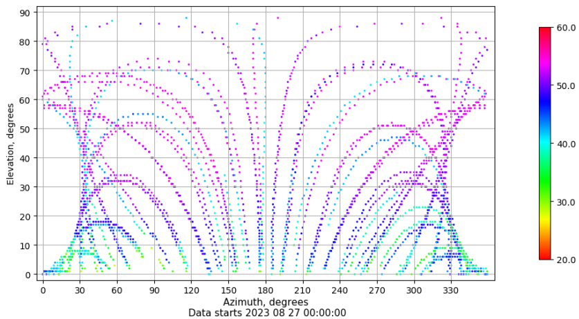
Azimuth-elevation plot for station SALA. Signal to Noise S1C Data file SALA00ESP_R_2023239.xtr
