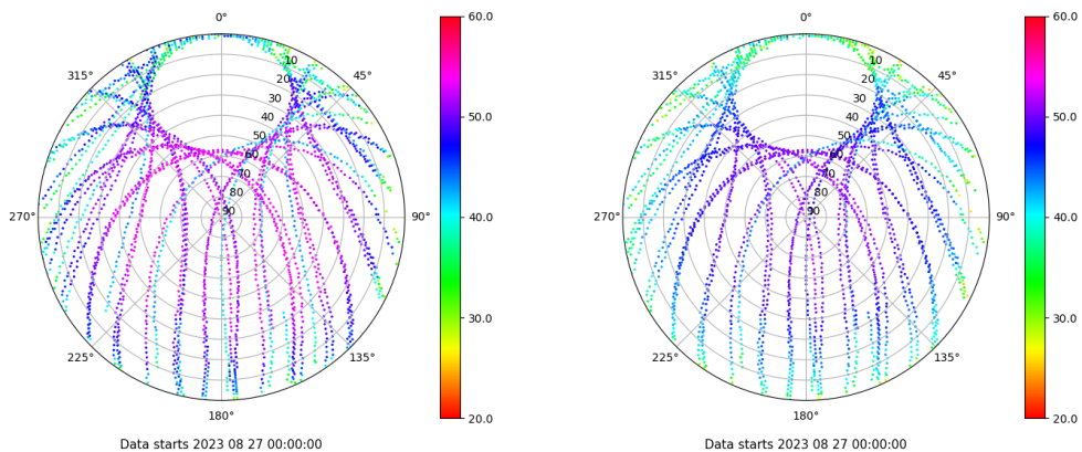
Skyplot for station SALA. Signal to Noise S1C Data file SALA00ESP_R_2023239.xtr Skyplot for station SALA. Signal to Noise S2P Data file SALA00ESP_R_2023239.xtr
