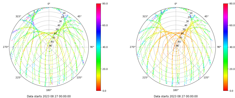
Skyplot for station SALA. Parameter M1C Data file SALA00ESP_R_2023239.xtr Skyplot for station SALA. Parameter M2P Data file SALA00ESP_R_2023239.xtr
