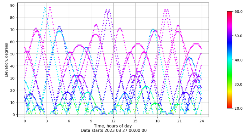
Time-elevation plot for station SALA. Signal to Noise S1C Data file SALA00ESP_R_2023239.xtr
